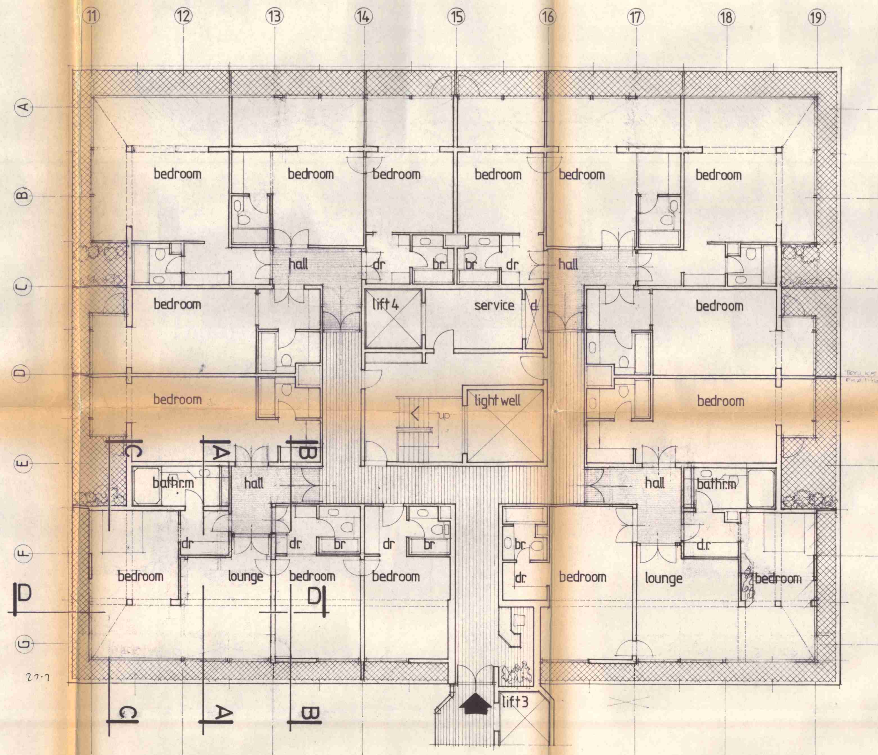
SEVENTH FLOOR PROPOSED BEDROOM RE-PLANNING
