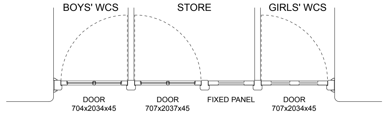
SECOND FLOOR GLAZED SCREEN
