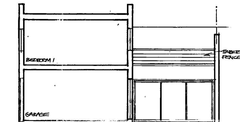
SIDE ELEVATION AND SECTION
