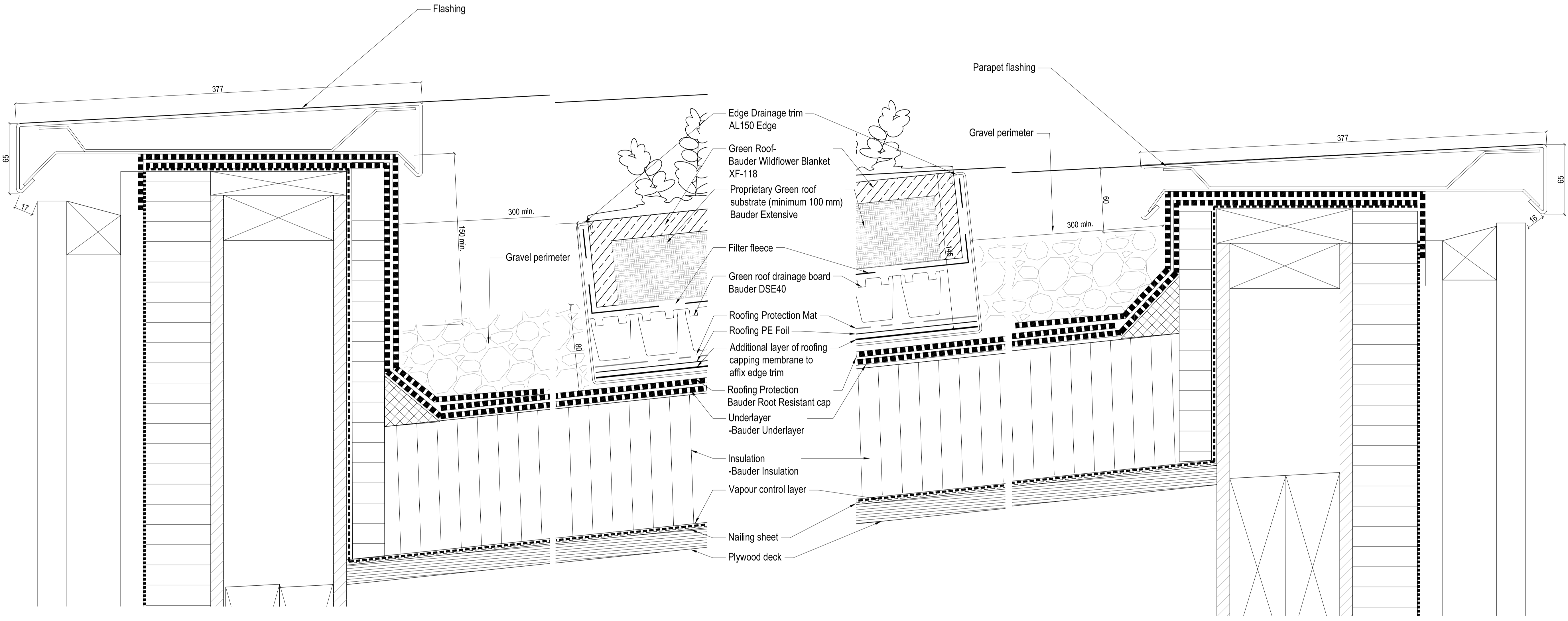
1 Green Roof Detail 1:2@A1
