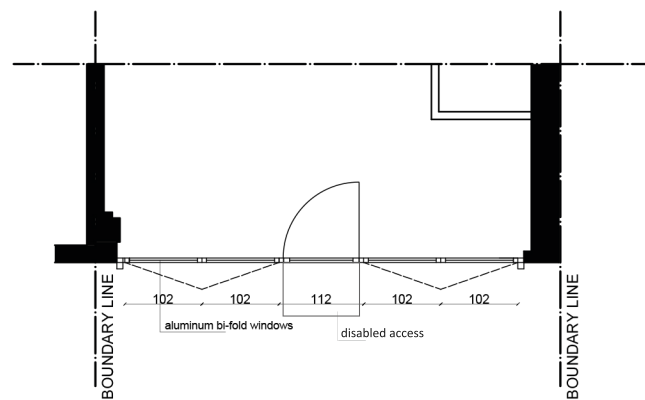
PROPOSED PLAN SCALE: 1/100 @ A3
