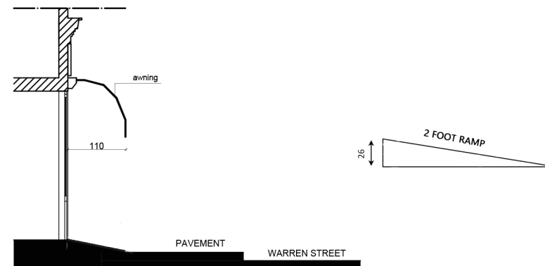
PROPOSED SECTION AA SCALE: 1/100 @ A3
