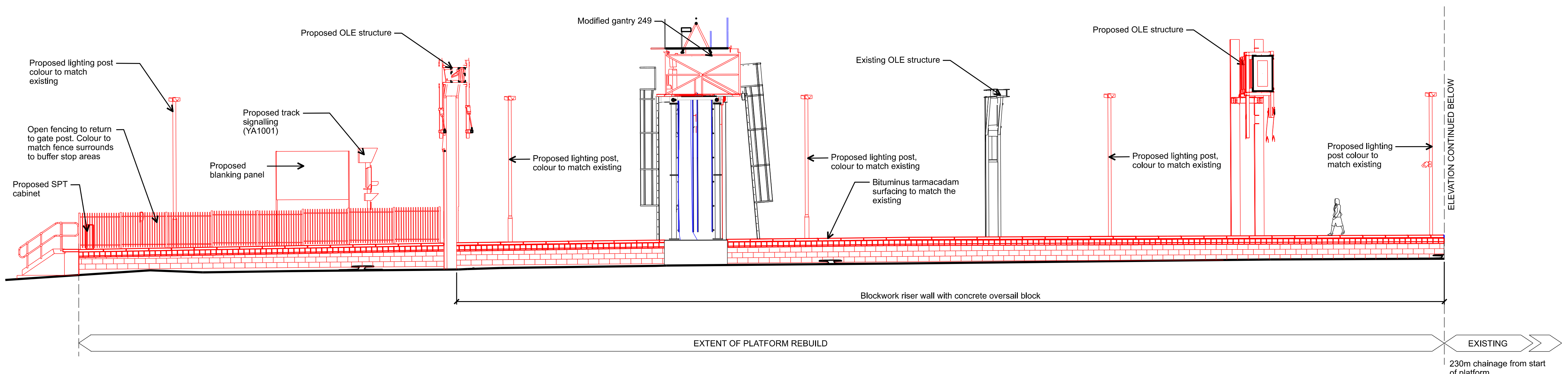
01 ELEVATION - PLATFORM 1 (1 OF 2)
