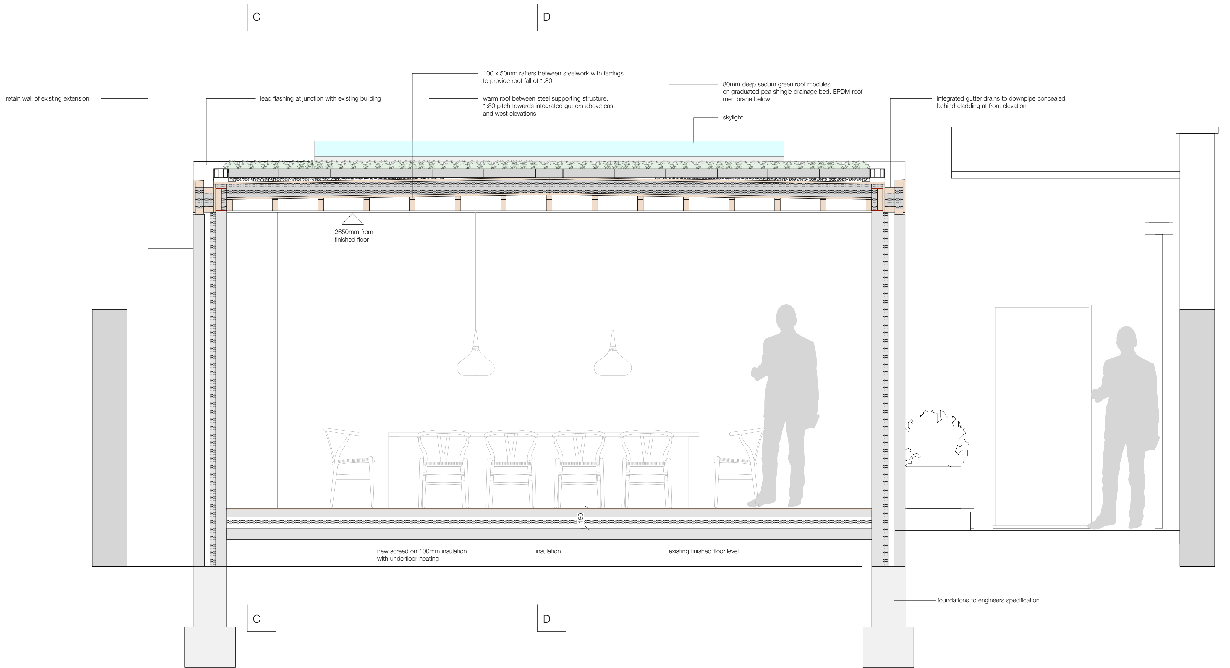
SECTION BB
