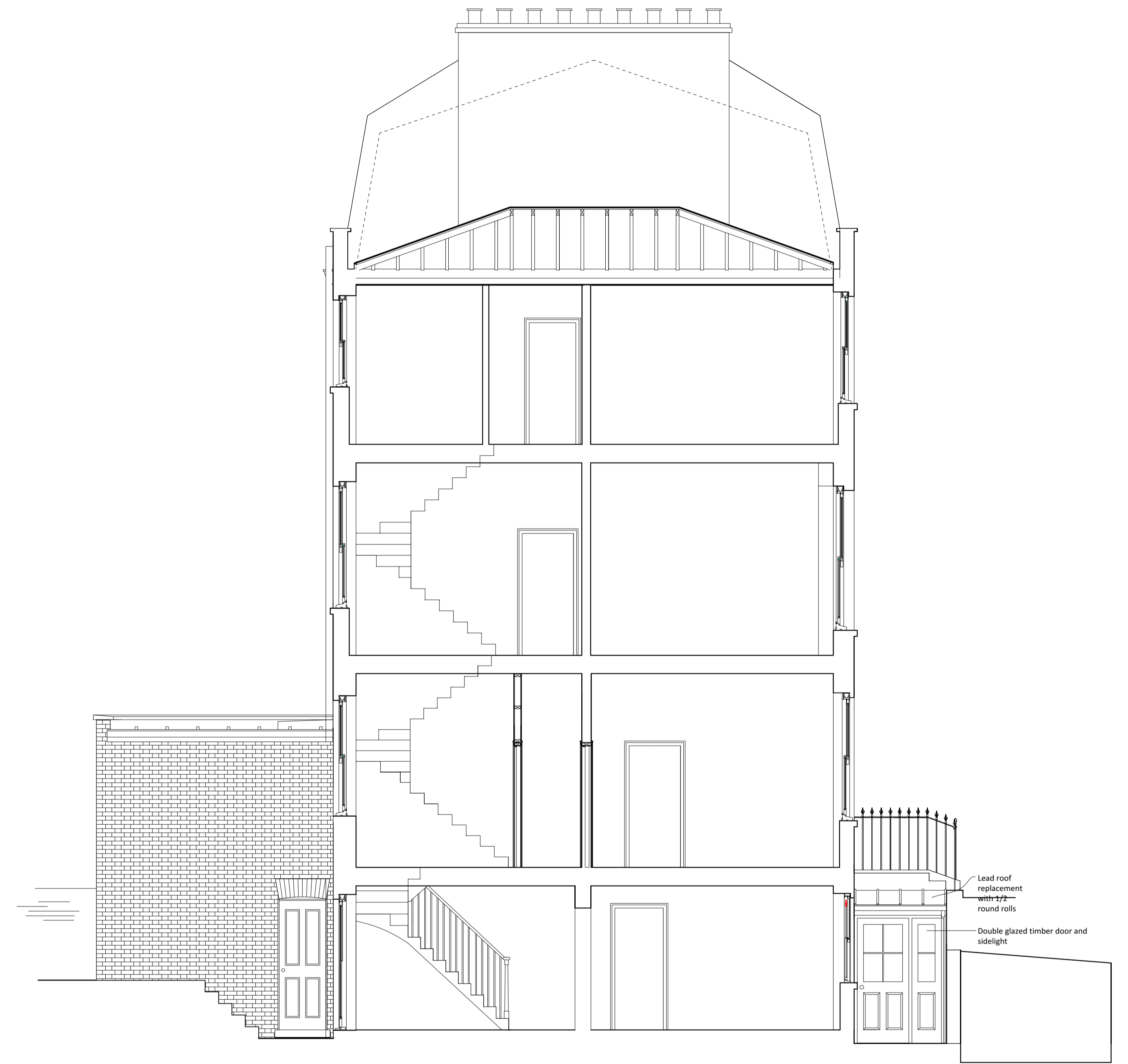
Section B-B
