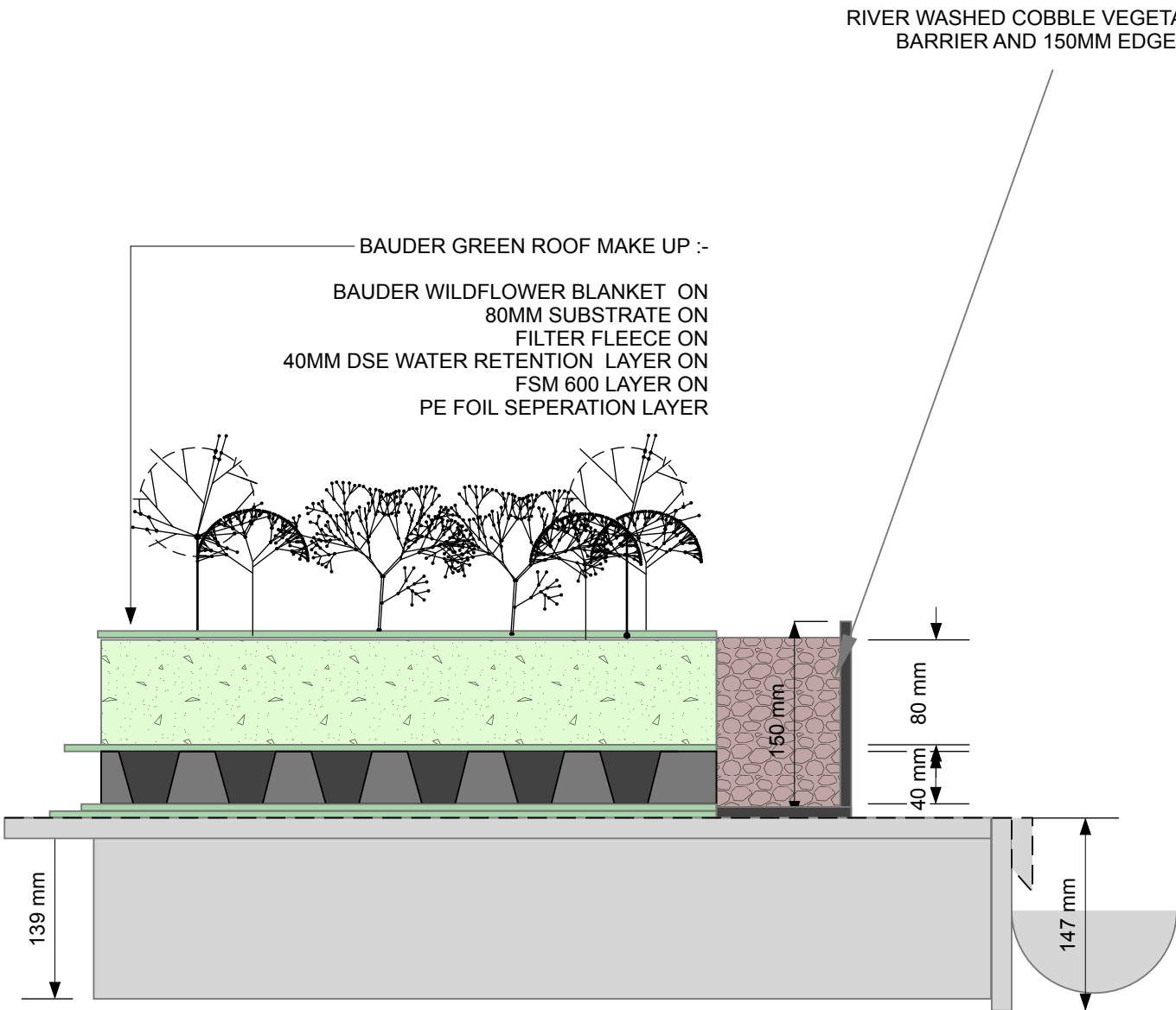
SECTION THROUGH GREEN ROOF 1:5
