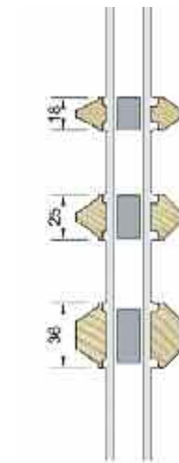
GLAZING BARS
