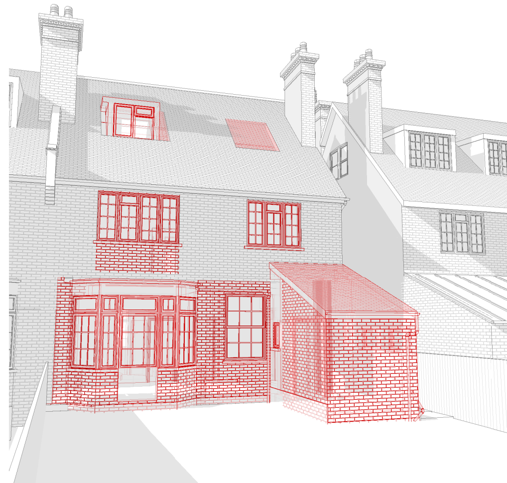
4 Demolition 3D View
