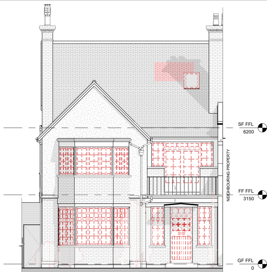
1 Existing Street Elevation 1 : 50
