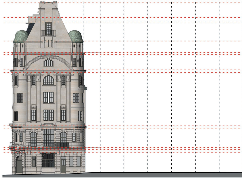
South elevation - initial idea
