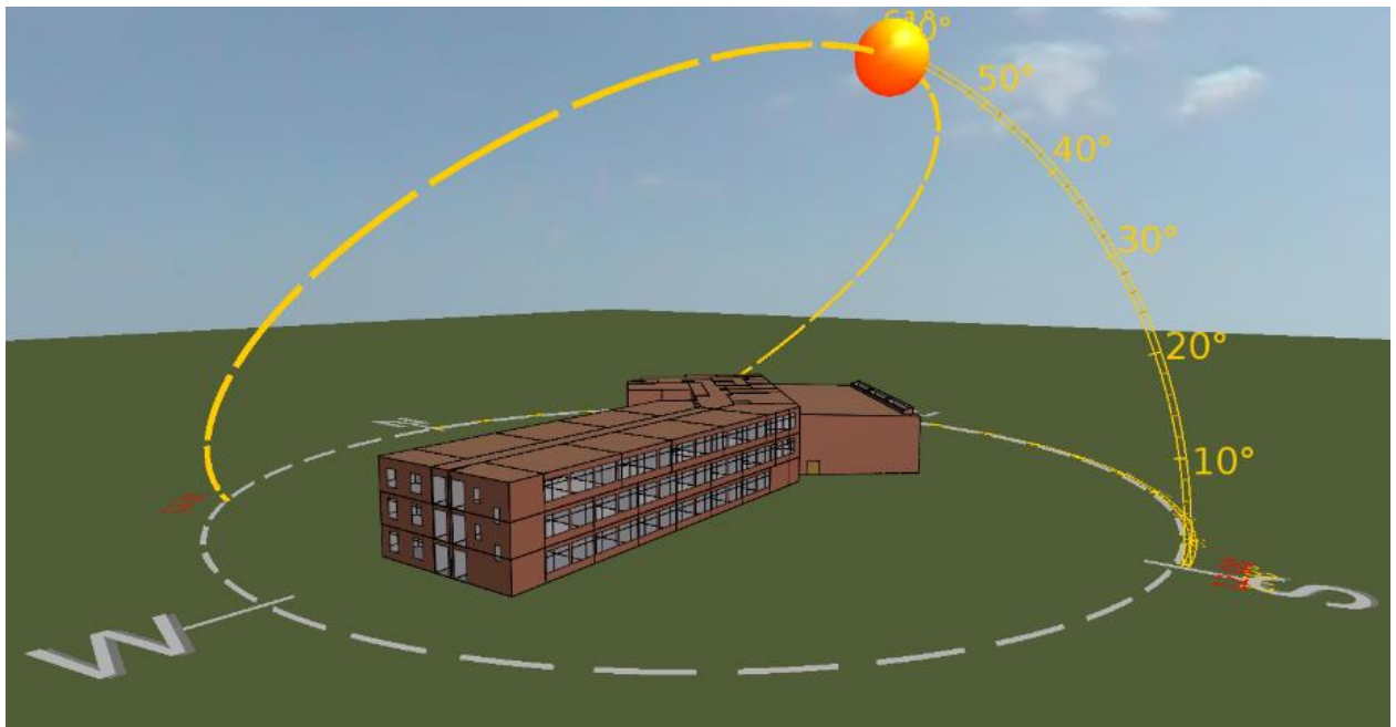
Parliament Hill School IES Model
