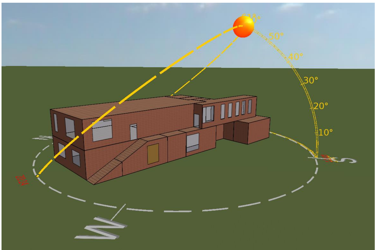
William Ellis School IES Model
