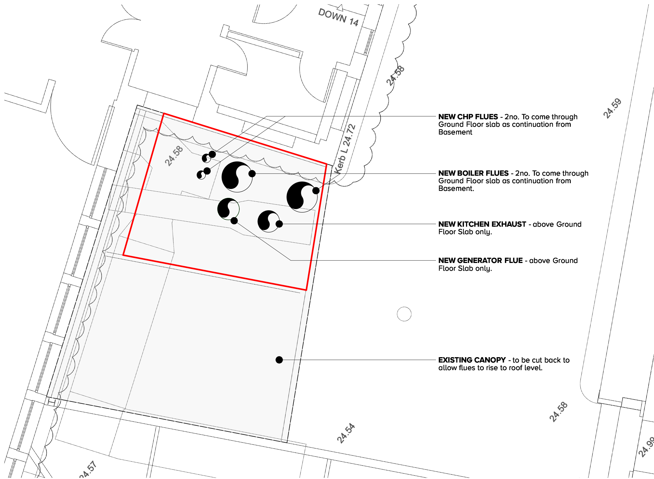
Part Ground Floor Plan - Proposed location for new flues
