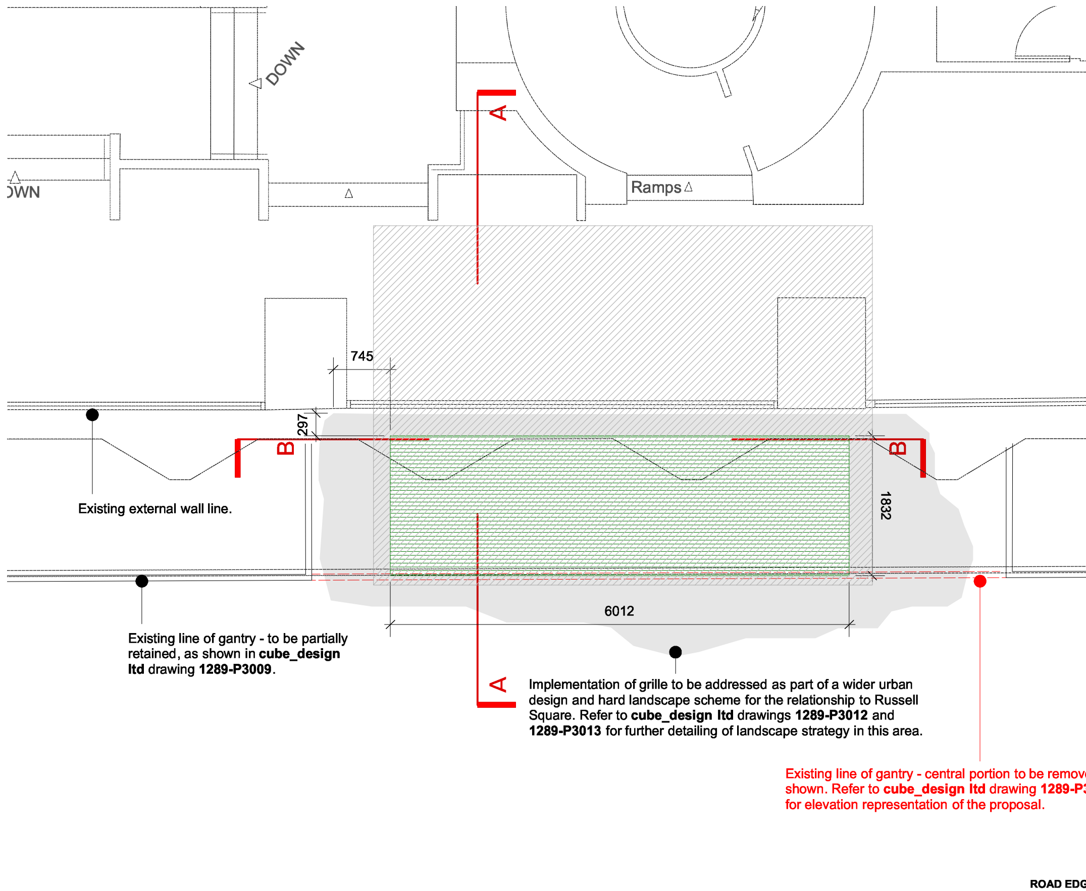
Part Ground Floor Plan - Proposed location for new transformer chamber
