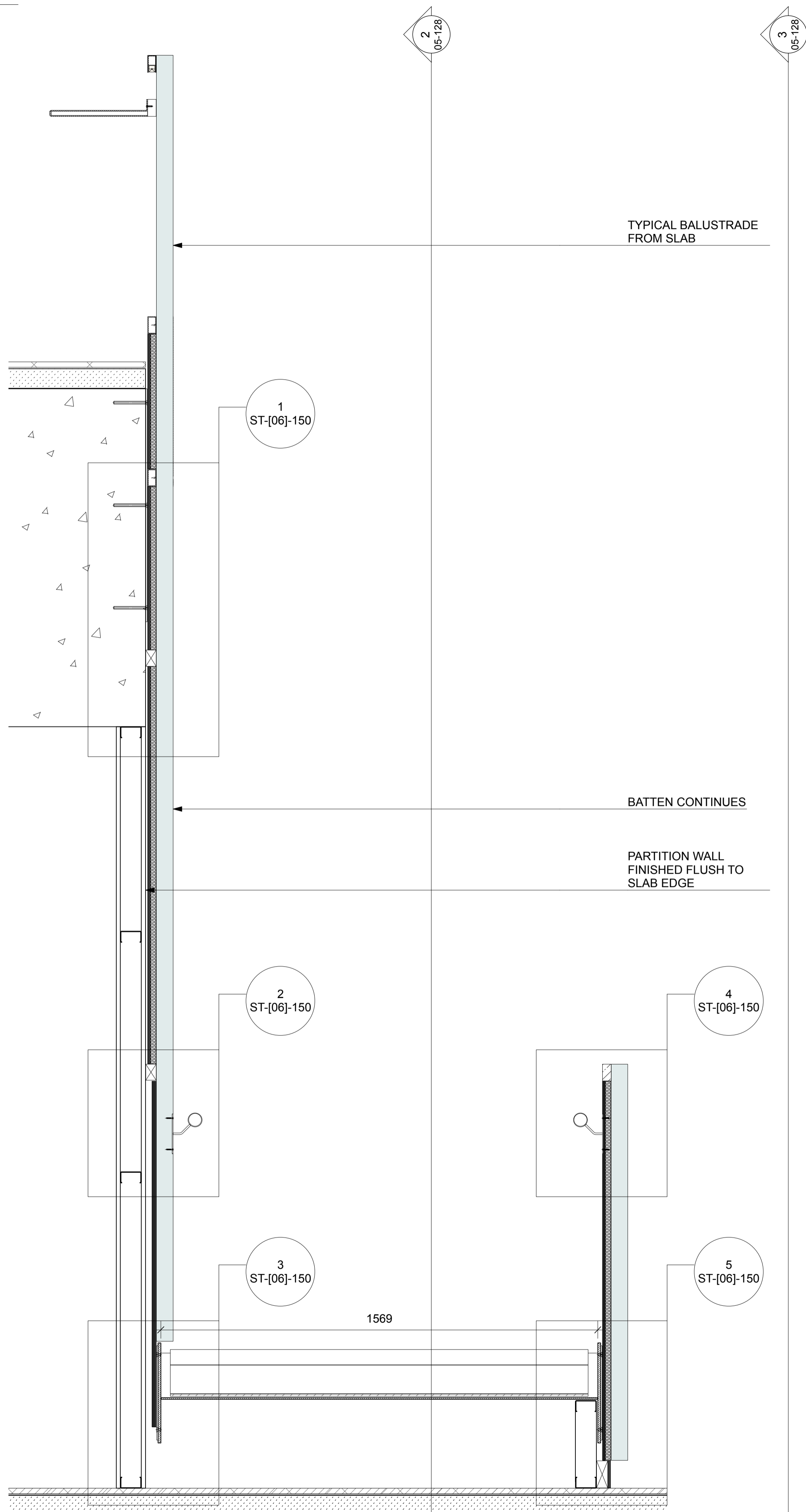
1 STAIR / SECTION TYPICAL Scale: 1:10
