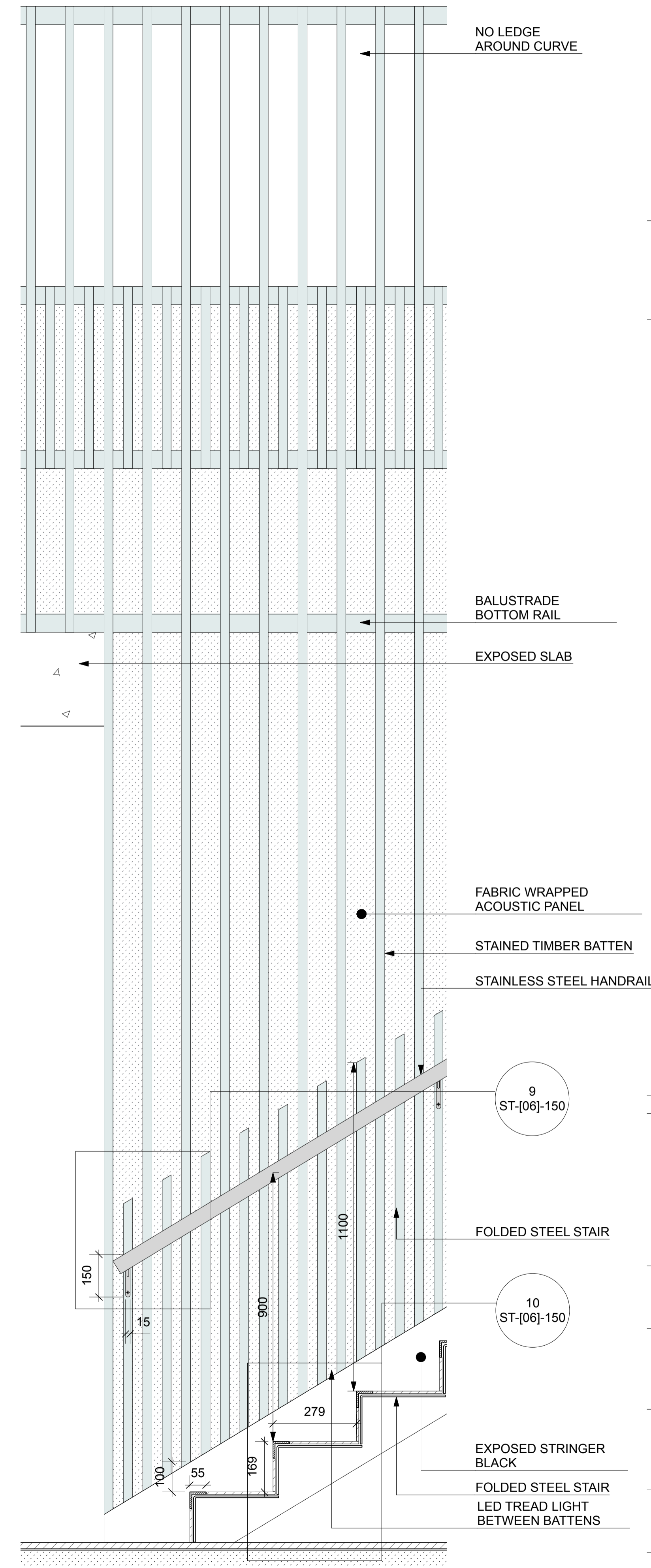
3 STAIR / SECTION TYPICAL Scale: 1:10
