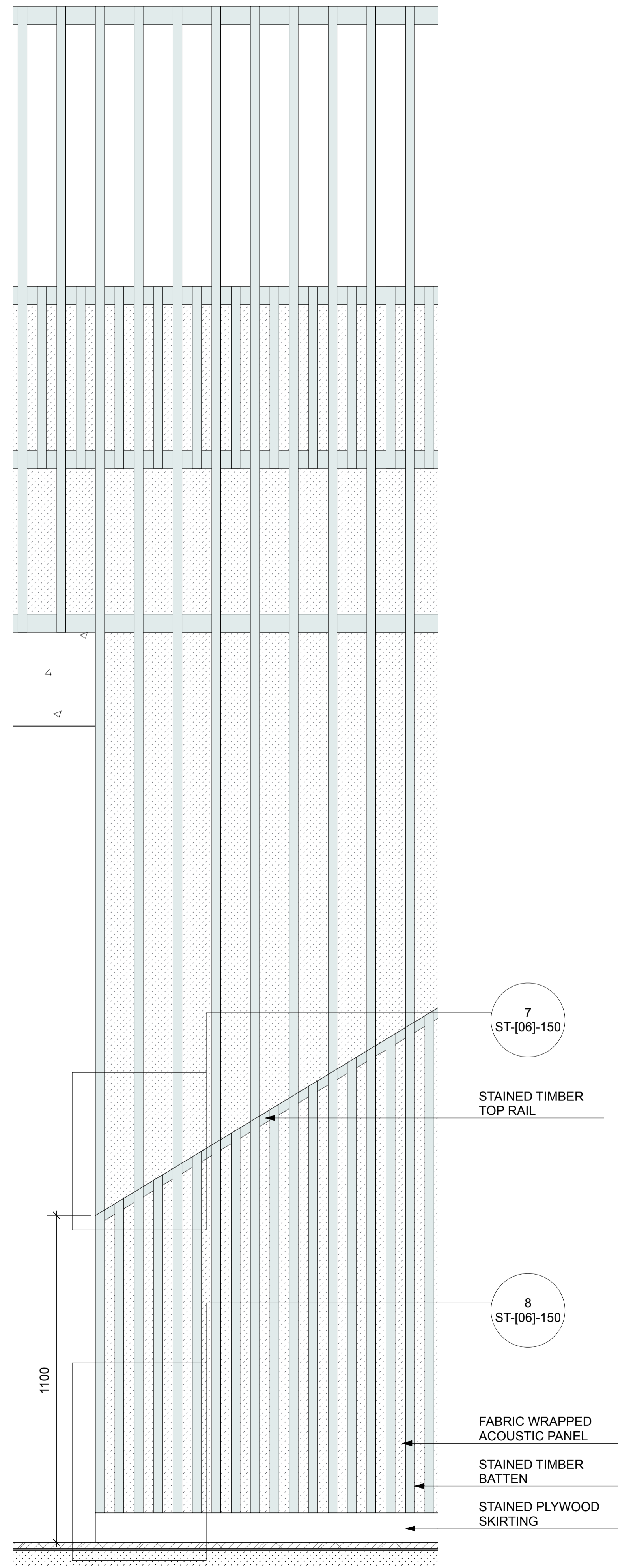
2 STAIR / ELEVATION TYPICAL Scale: 1:10
