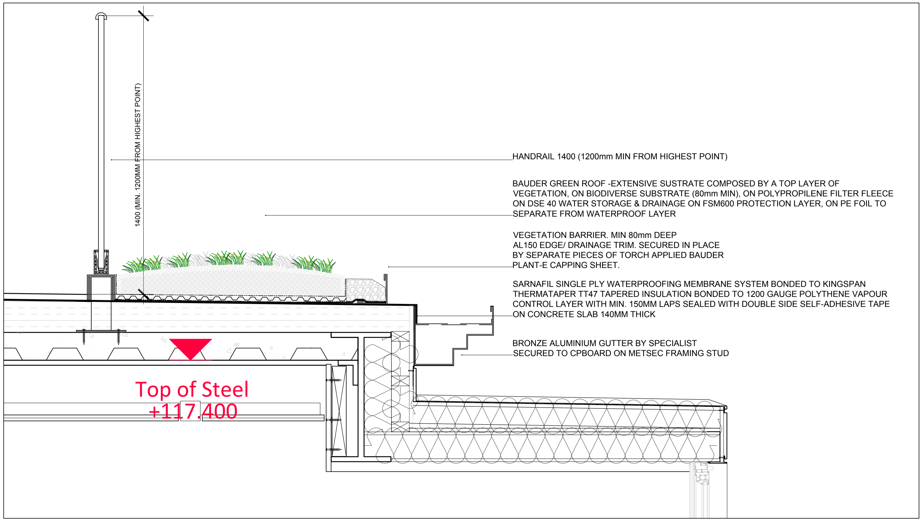
DINNING HALL PERIMETER ROOF DETAIL
