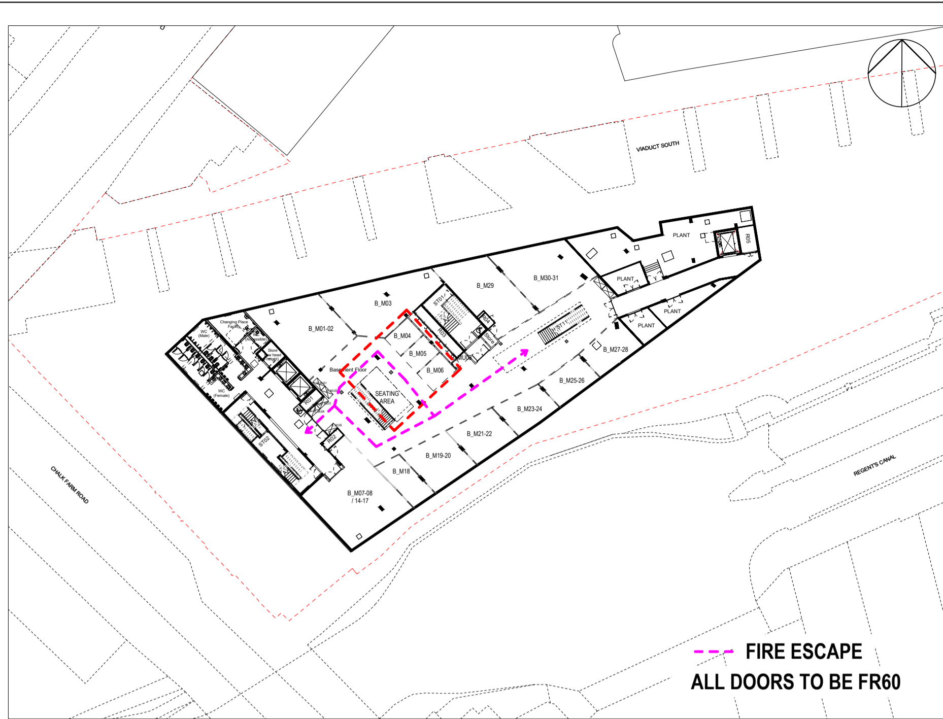
UPPER LOCK _ BASEMENT PLAN SCALE 1:500
