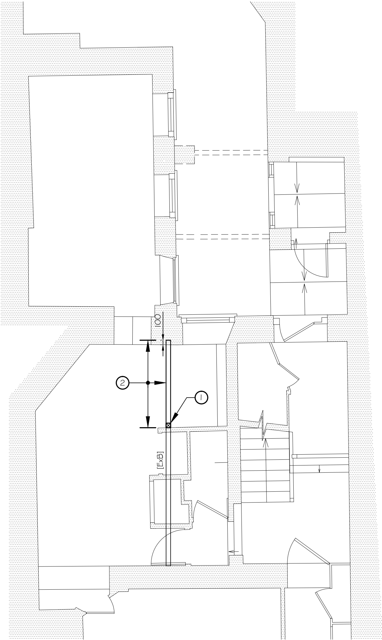
Basement Plan Showing Timber Remedial Works Requirements
