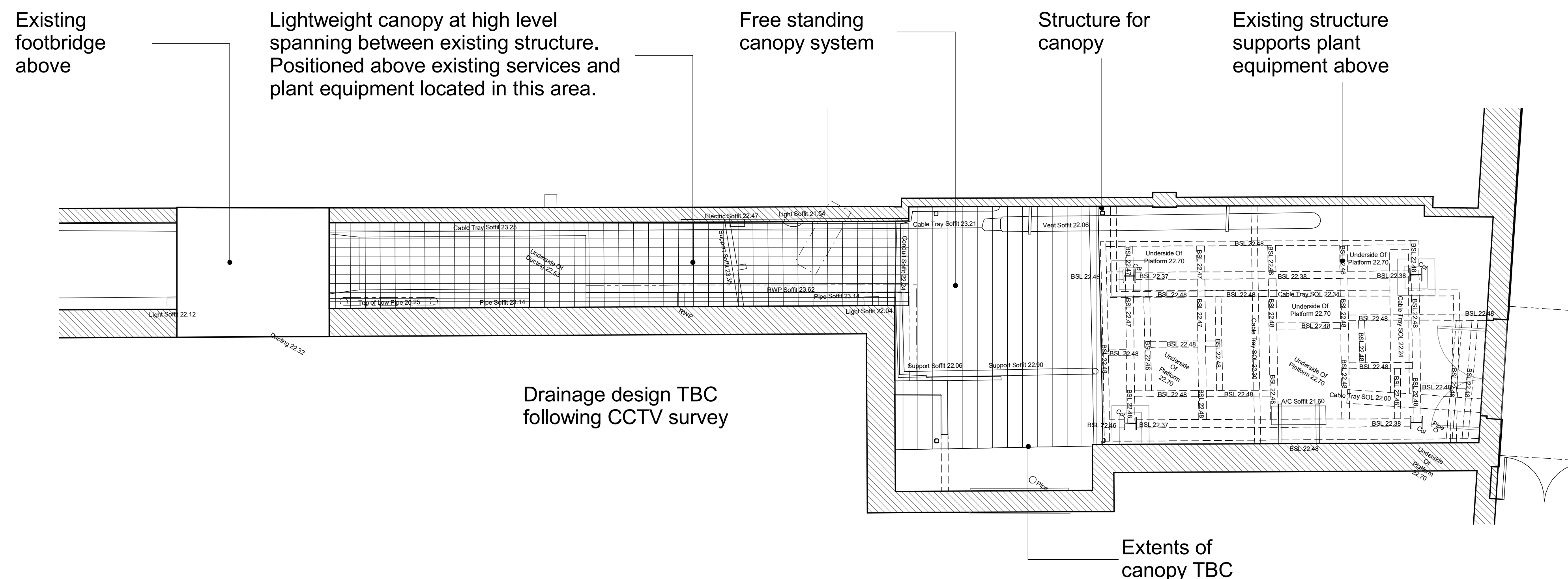
Proposed Dirty Corridor - Roof Plan
