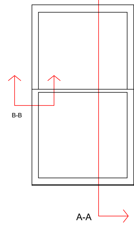
Secondary glazing Section A-A
