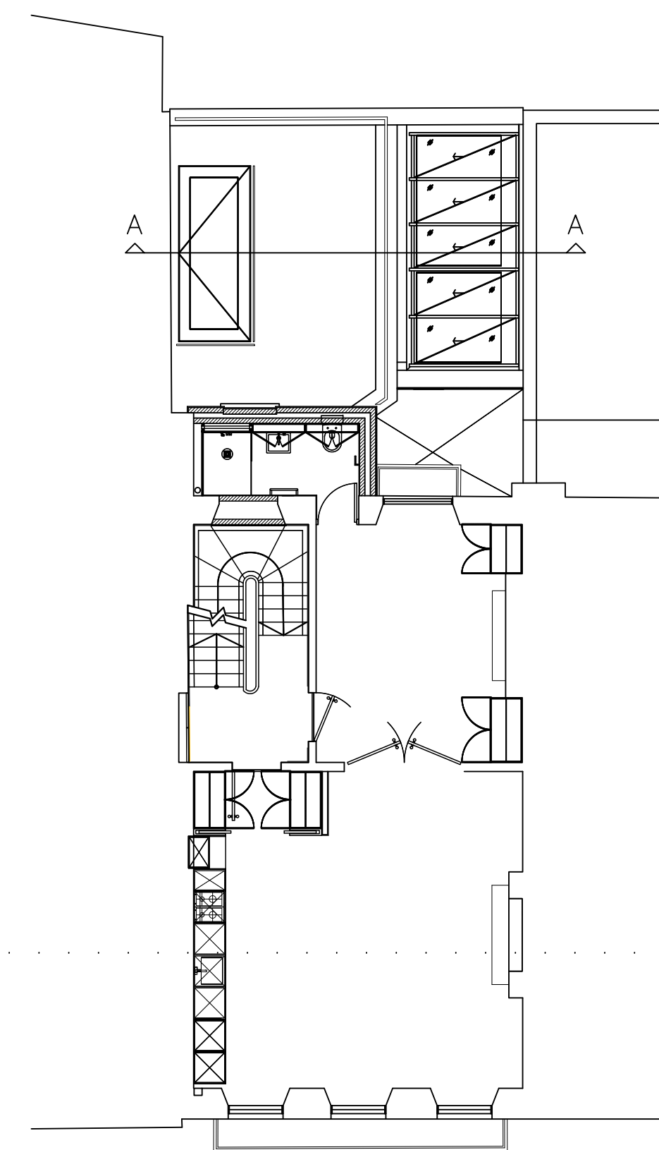
Proposed First Floor – 1:10
