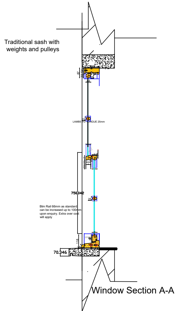
Window Section A-A
