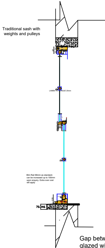
Window Section A-A
