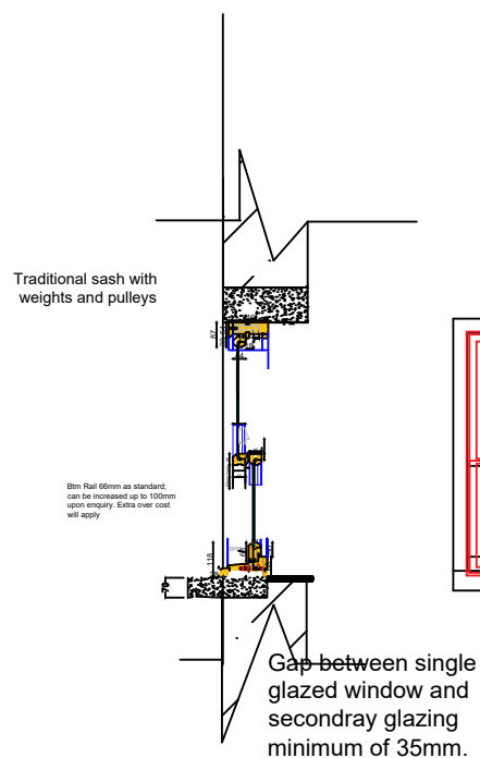
Window Section A-A
