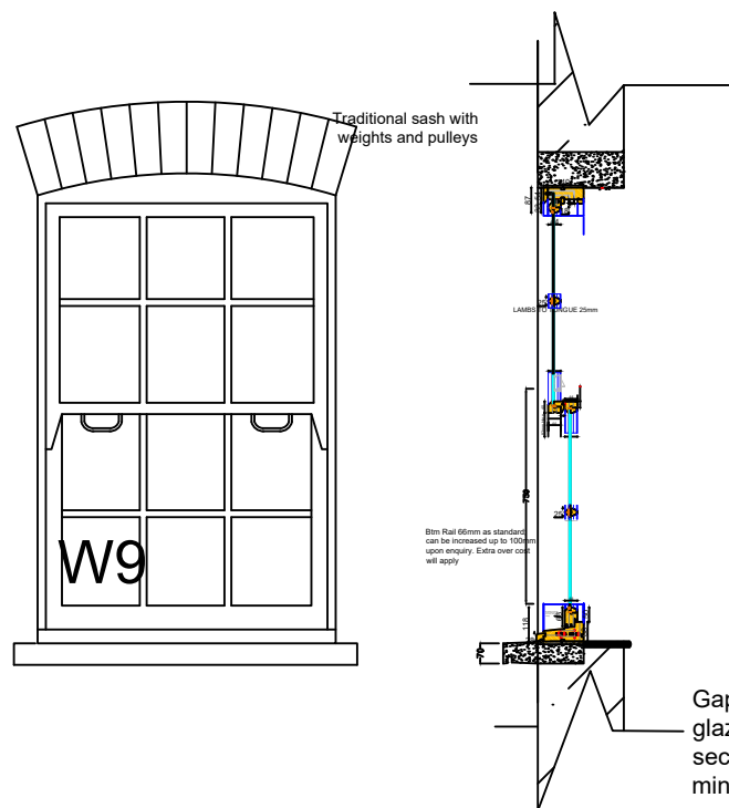
Window Section A-A
