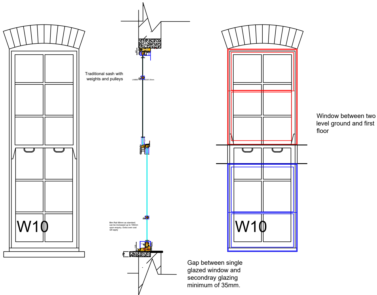
Window Section A-A
