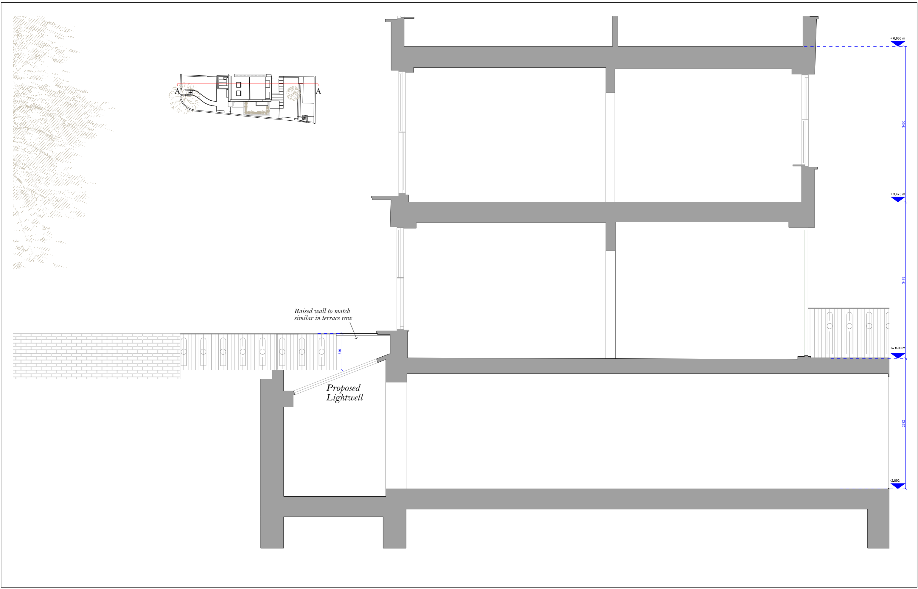
Proposed_Section AA
