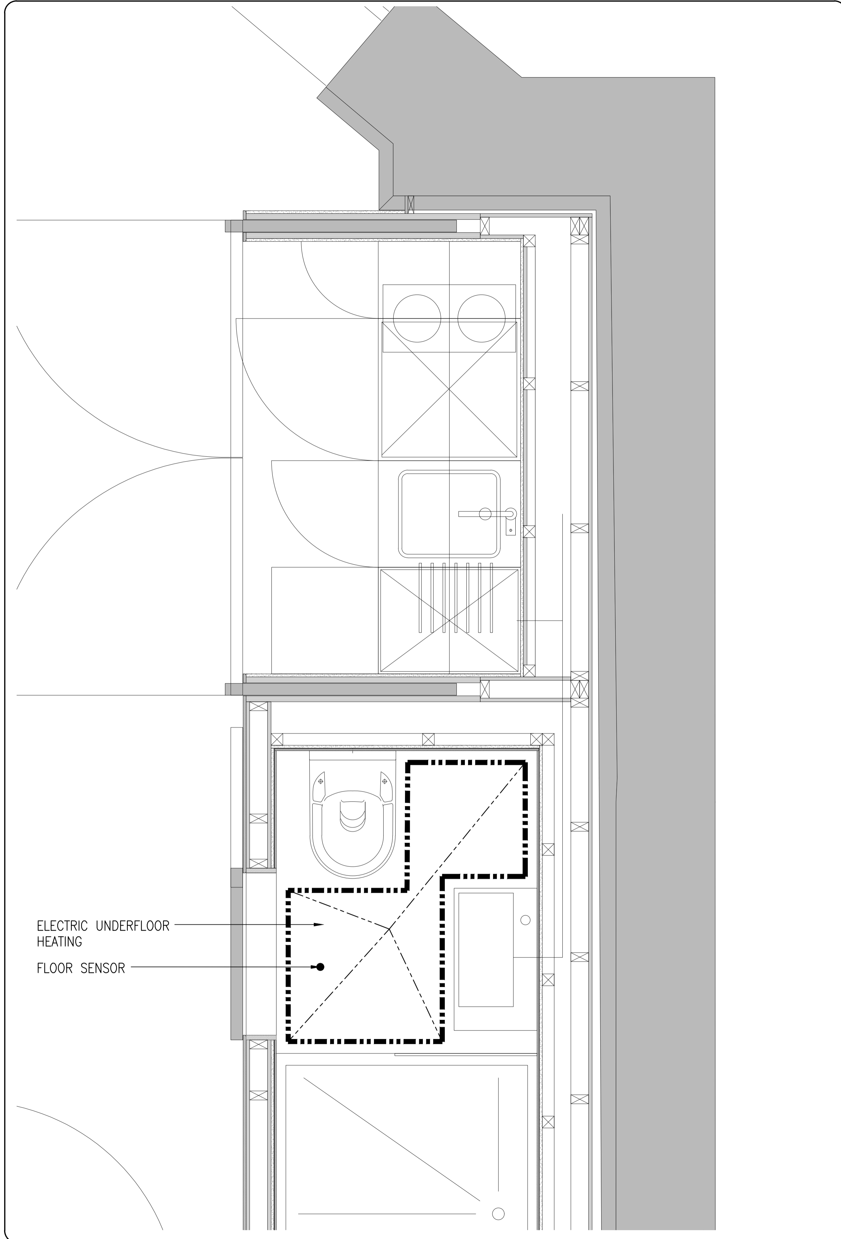
PLAN VIEW
