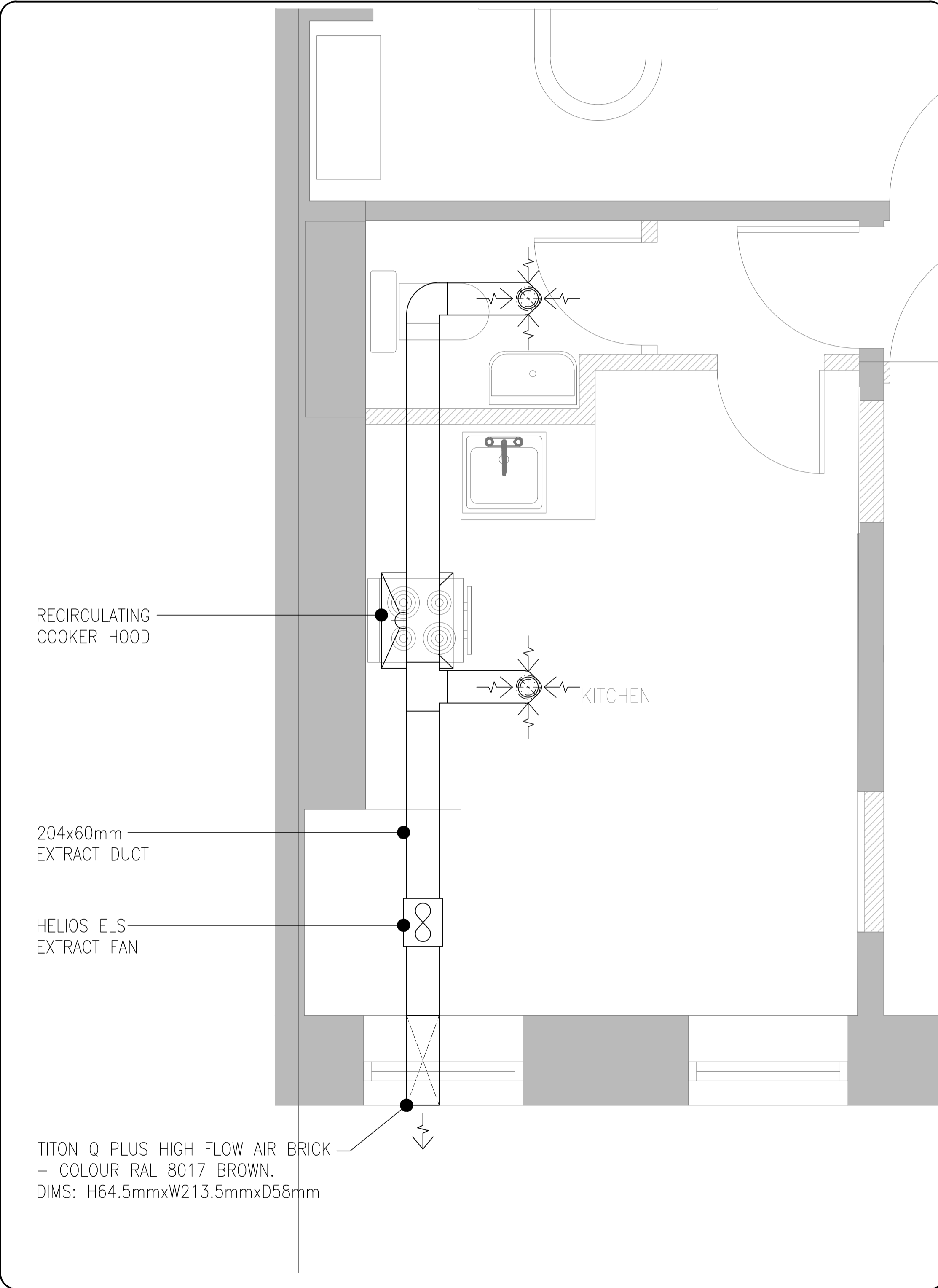
SECOND FLOOR DUPLEX DETAIL
