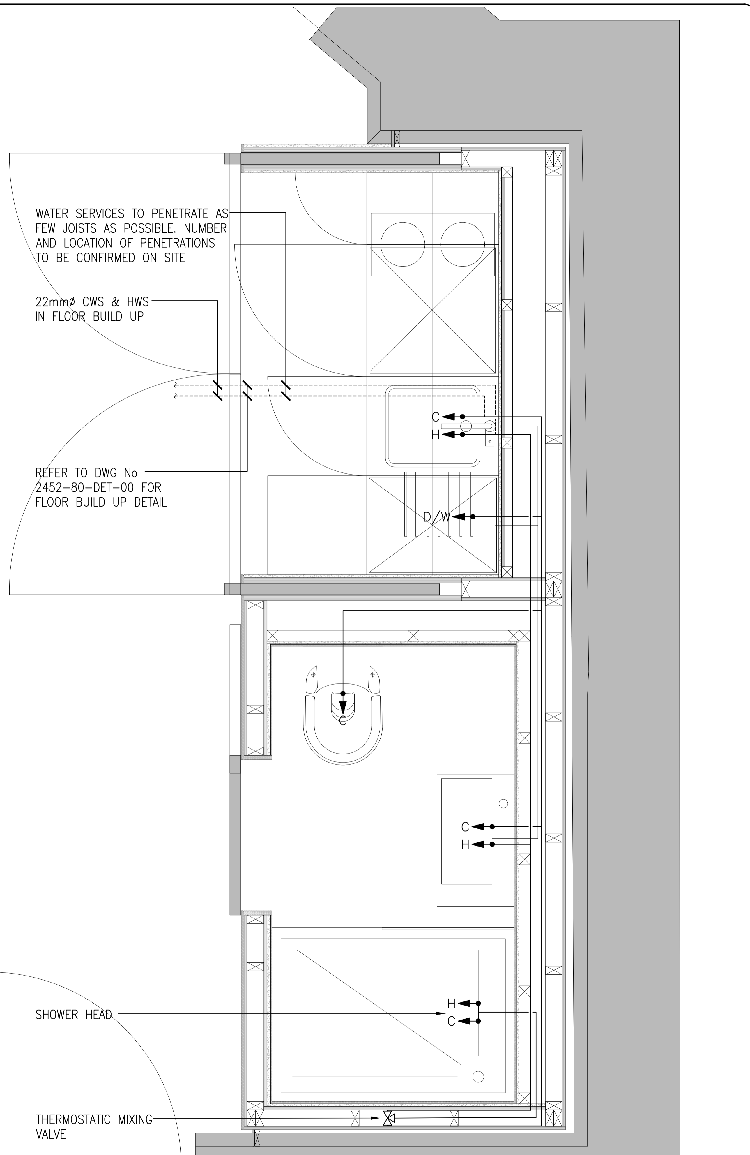
PLAN VIEW
