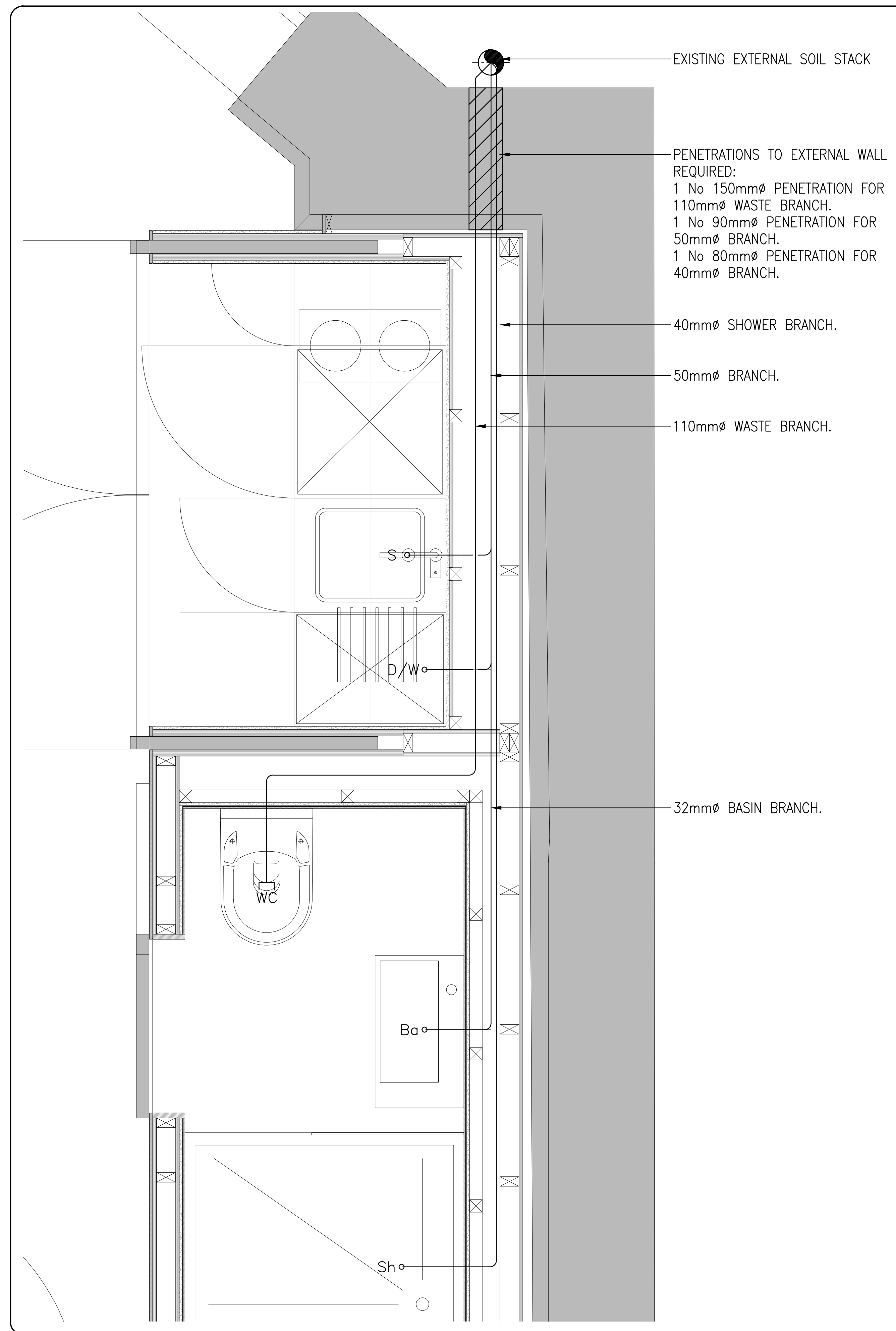
PLAN VIEW
