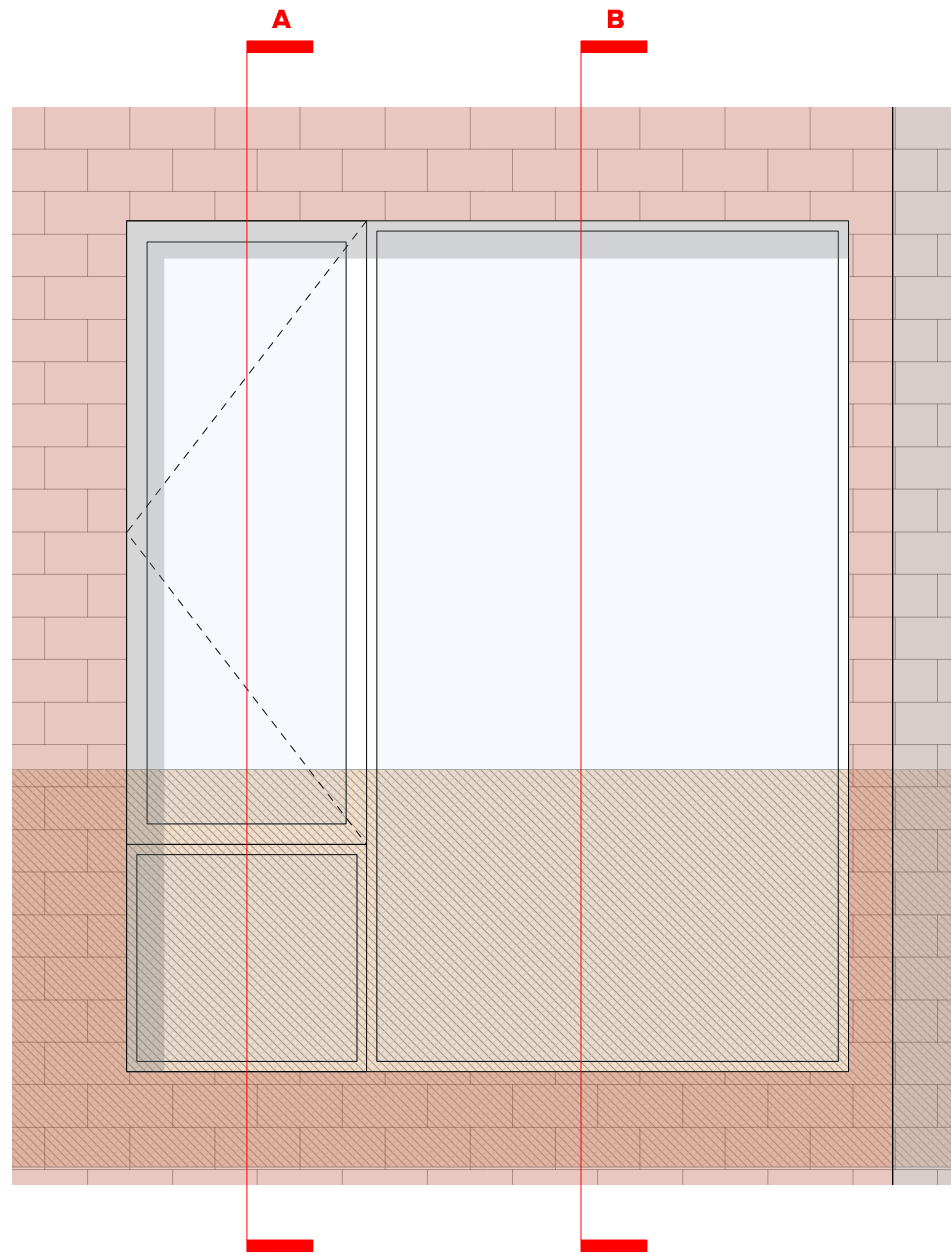
WINDOW ELEVATION Full Height Bedroom - Window Type 07a (07b mirrored)
