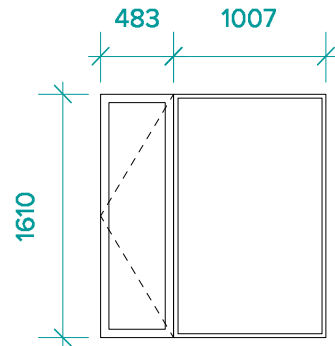
SO Type 03a (V Bedroom) Estimated Quantity: 182
