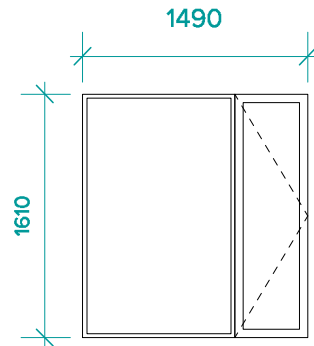
SO Type 03b (V Bedroom) Estimated Quantity: 203
