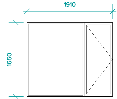
SO Type 06b (Flat Bedroom) Estimated Quantity: 70
