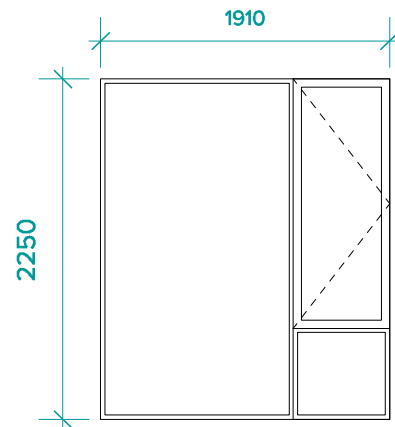
SO Type 07b (Full Height Bedroom) Estimated Quantity: 28
