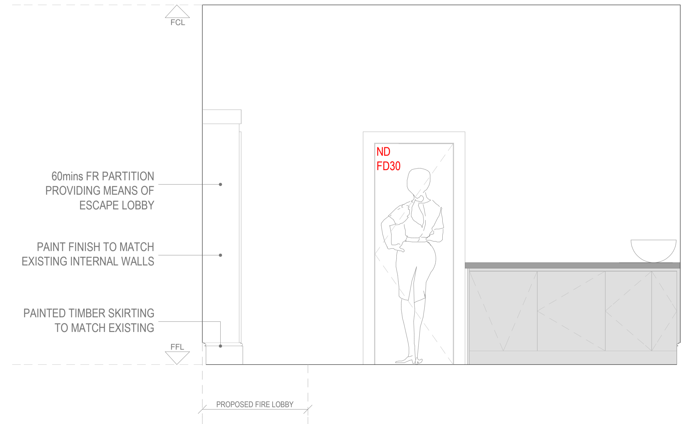
PROPOSED LOBBY ELEVATION A @ 1 : 20
