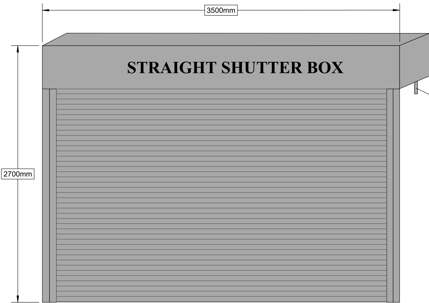
FRONT ELEVATION
