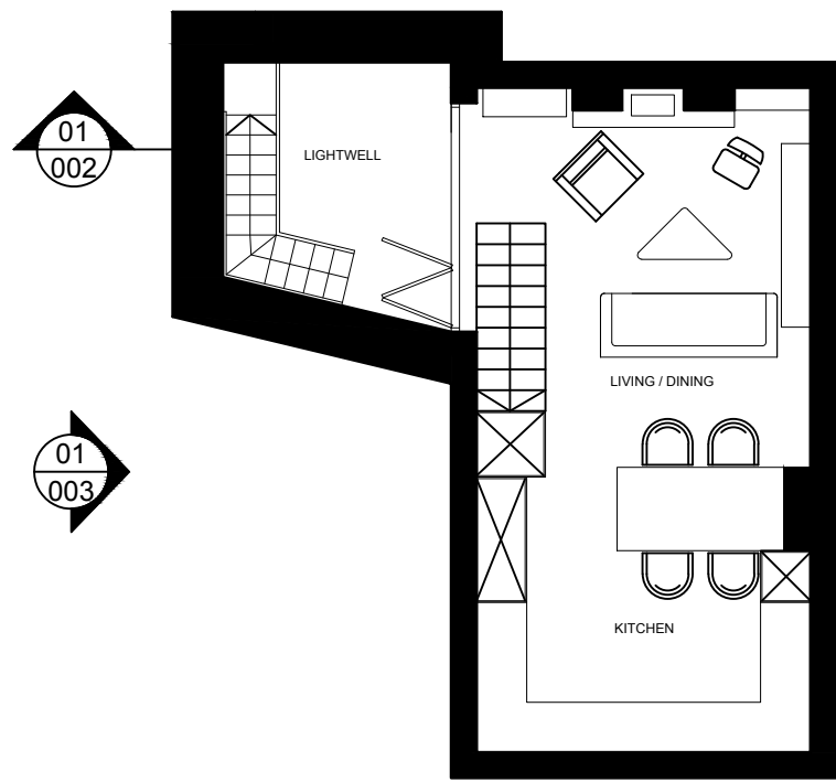
01 Lower Ground Floor 1:100
