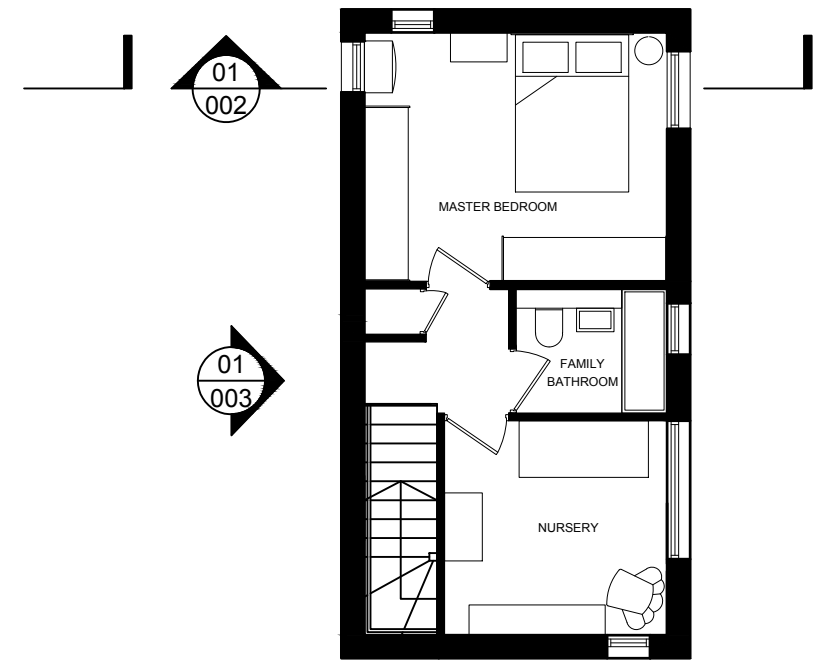
03 First Floor 1:100
