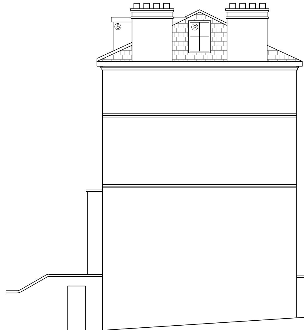
SIDE ELEVATION
