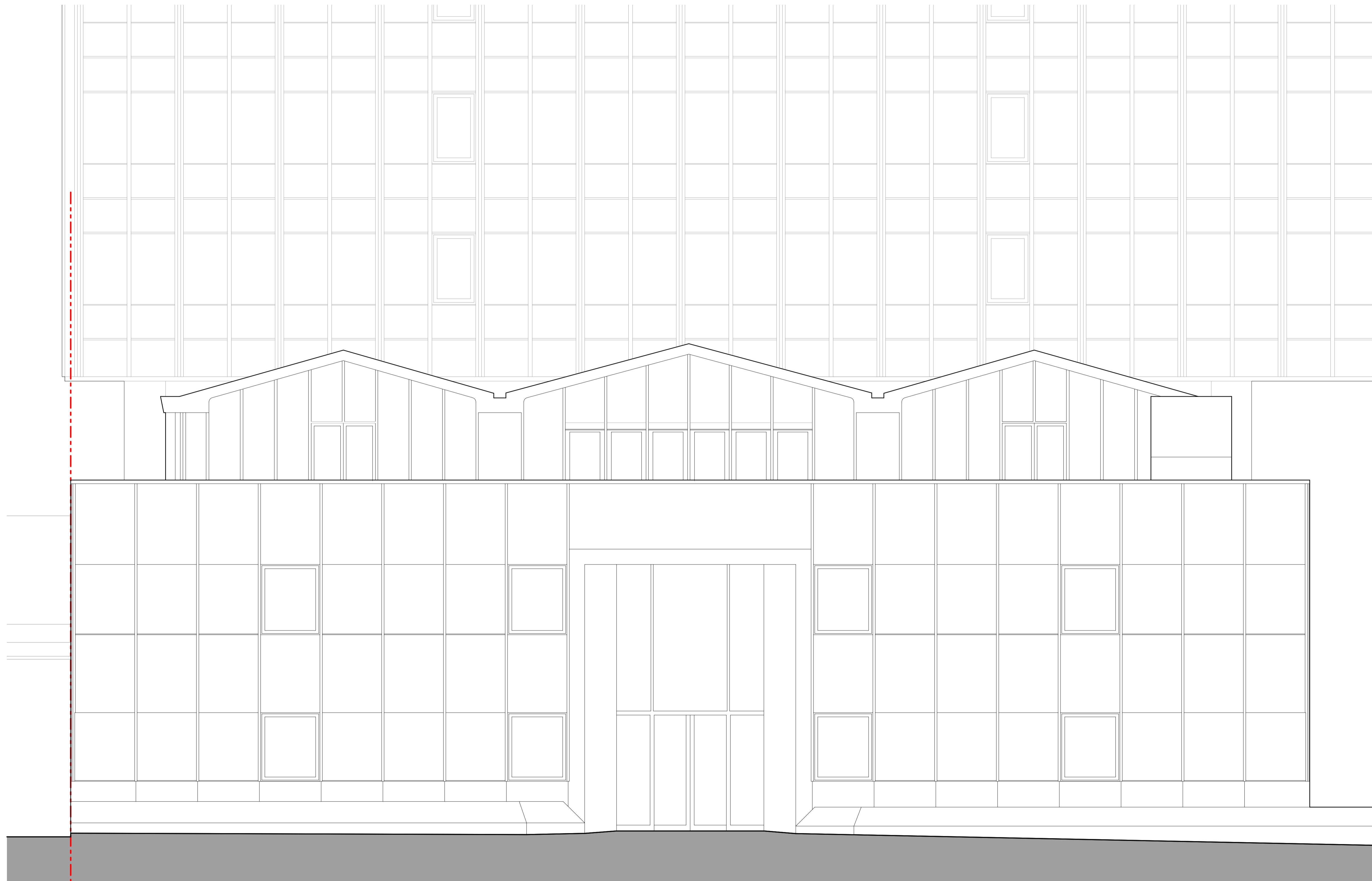
South elevation
