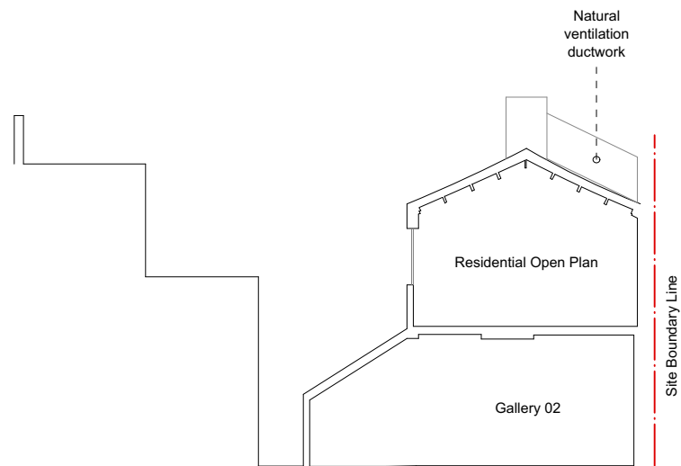
3 Section CC
