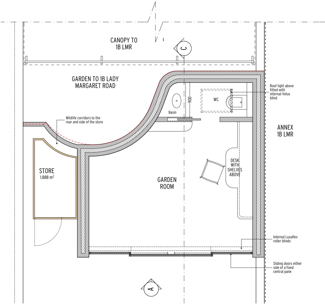
PROPOSED PLAN - 1:50 @ A3
