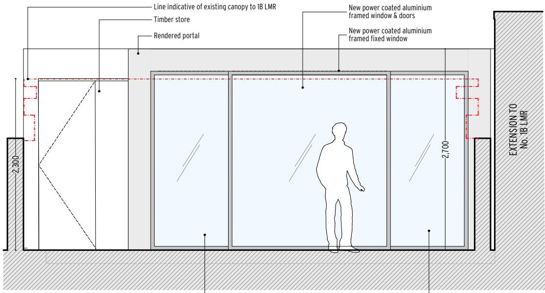
PROPOSED ELEVATION A - 1:50 @ A3
