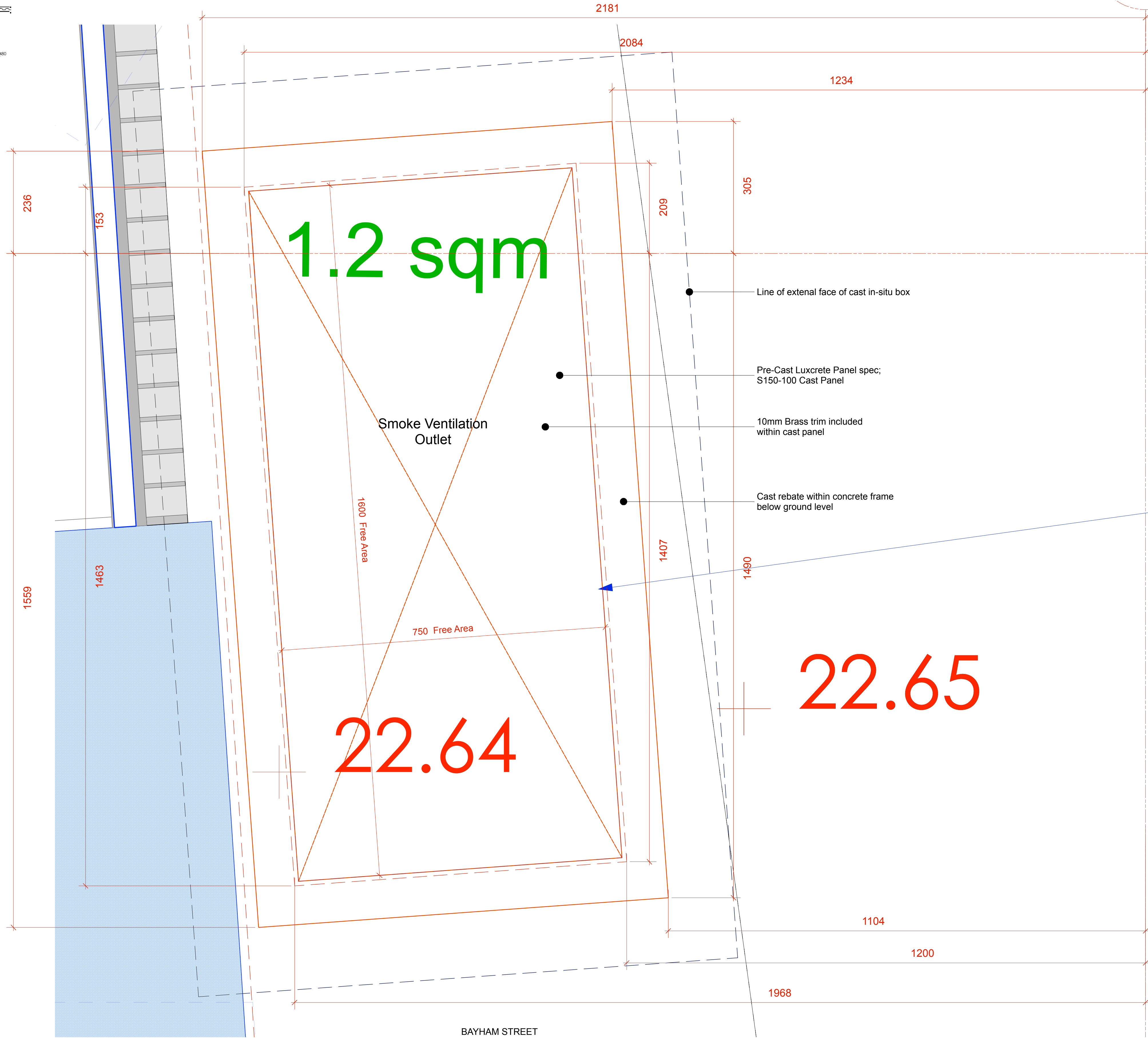
1 Detail 01 - Pavement opening Scale: 1:5
