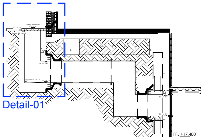
2 Detailed Section Scale: 1:100
