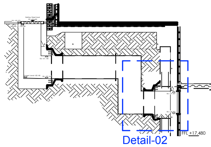
1 Detailed Section Scale: 1:100
