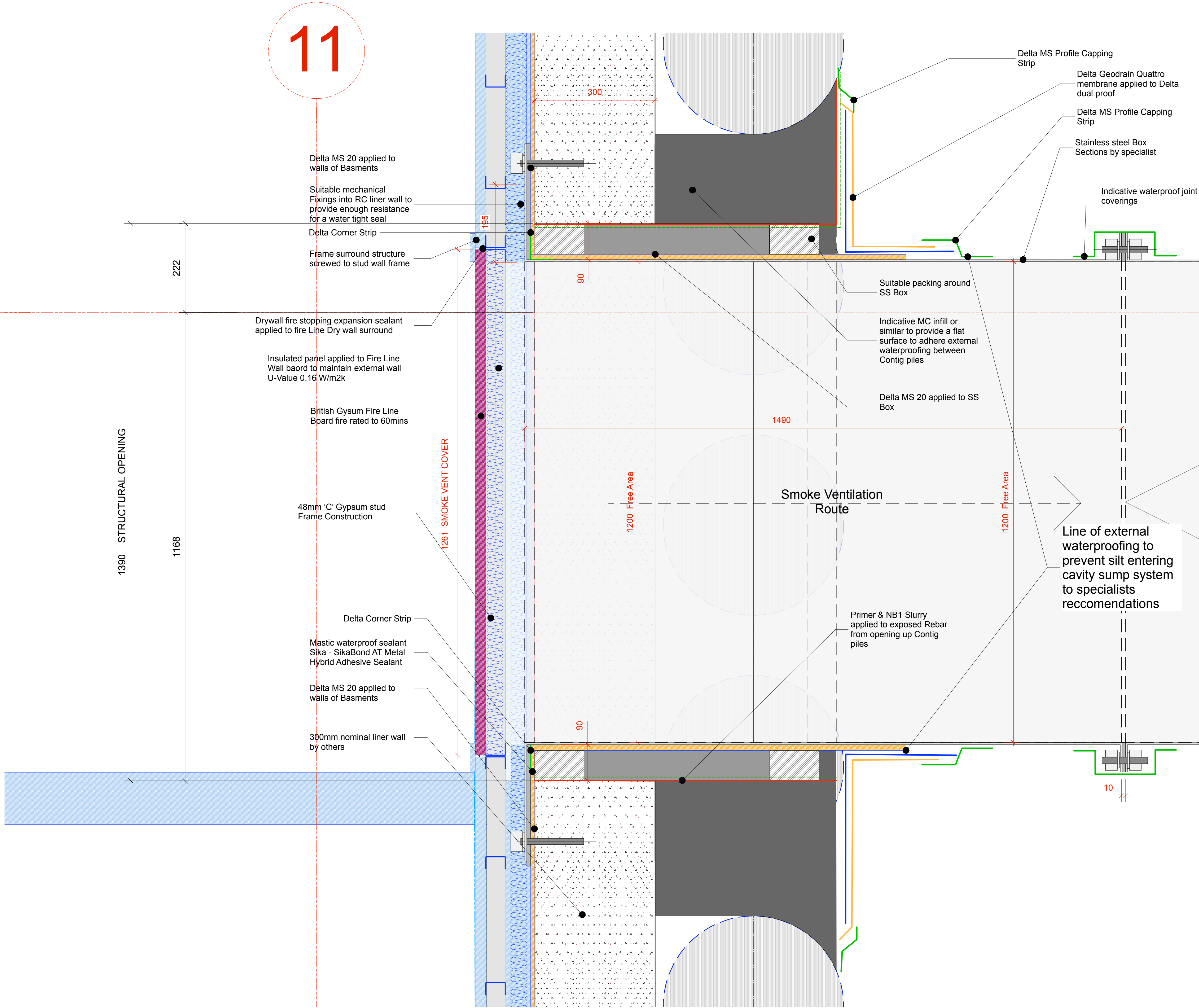
2 Detail 02 - Liner wall opening Scale: 1:5
