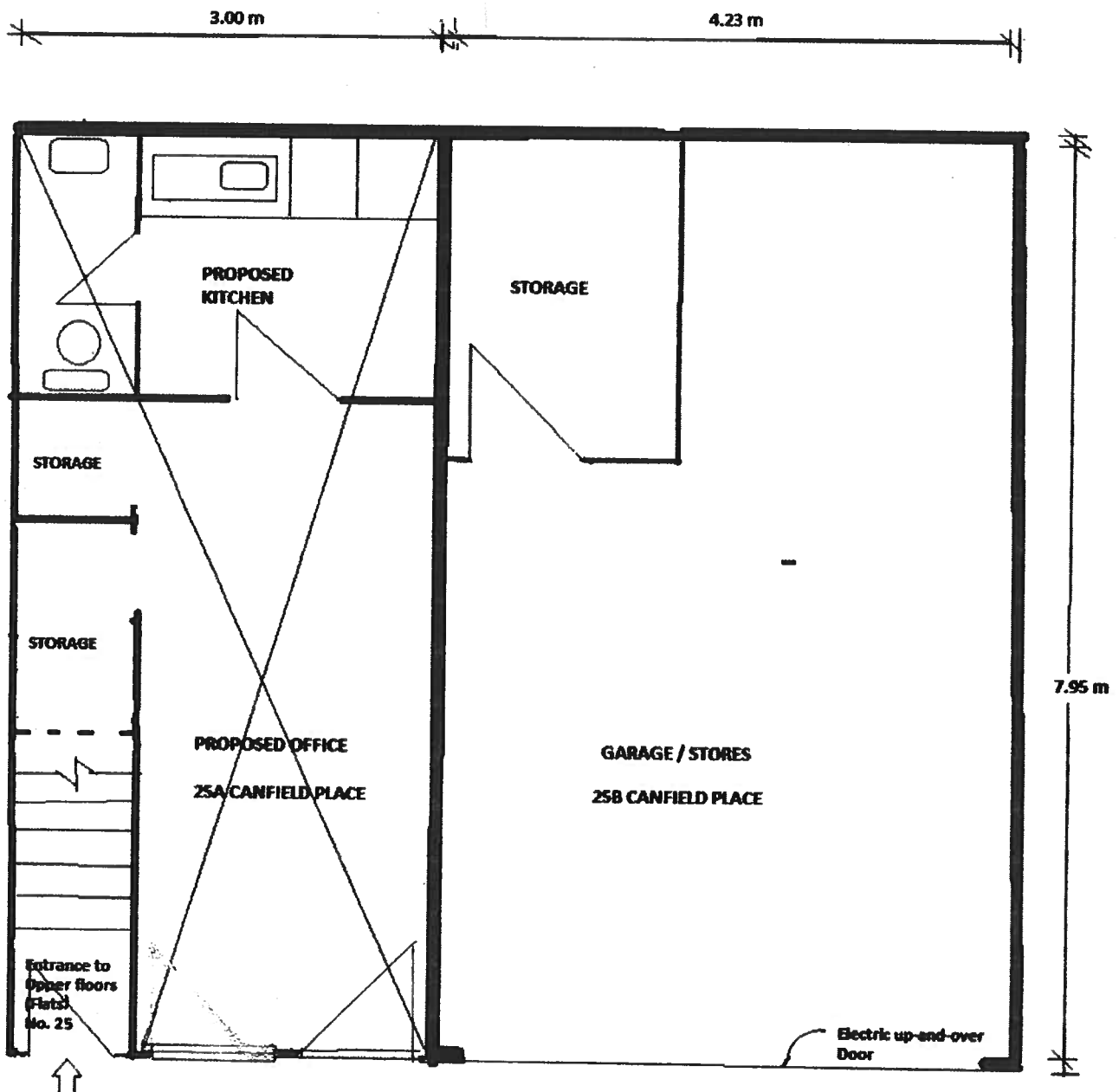
GROUND FLOOR PLAN - 25 CANFIELD PLACE
