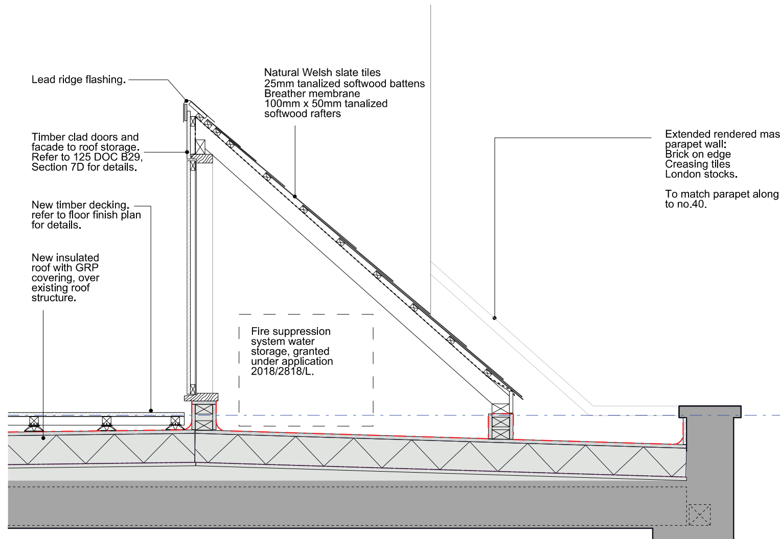
Short section through proposed roof
