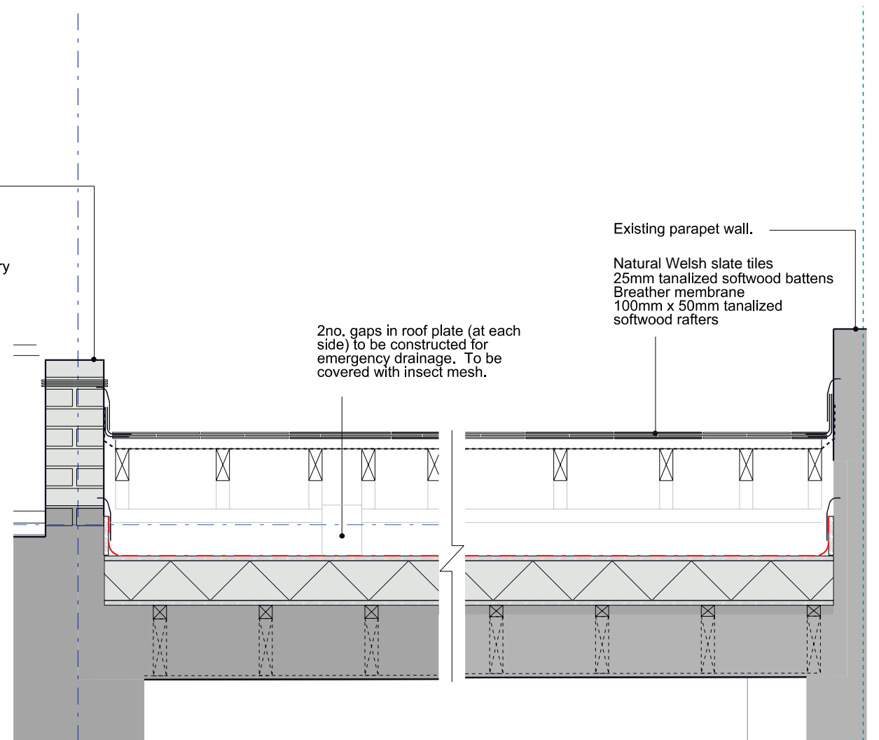
Long section through proposed roof.
