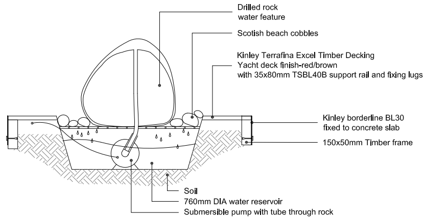
3 Section Through Water Feature TS-DT-001
