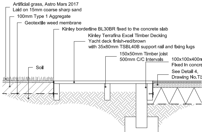
2 Section Through Artificial Grass - Timber Decking TS-DT-001
