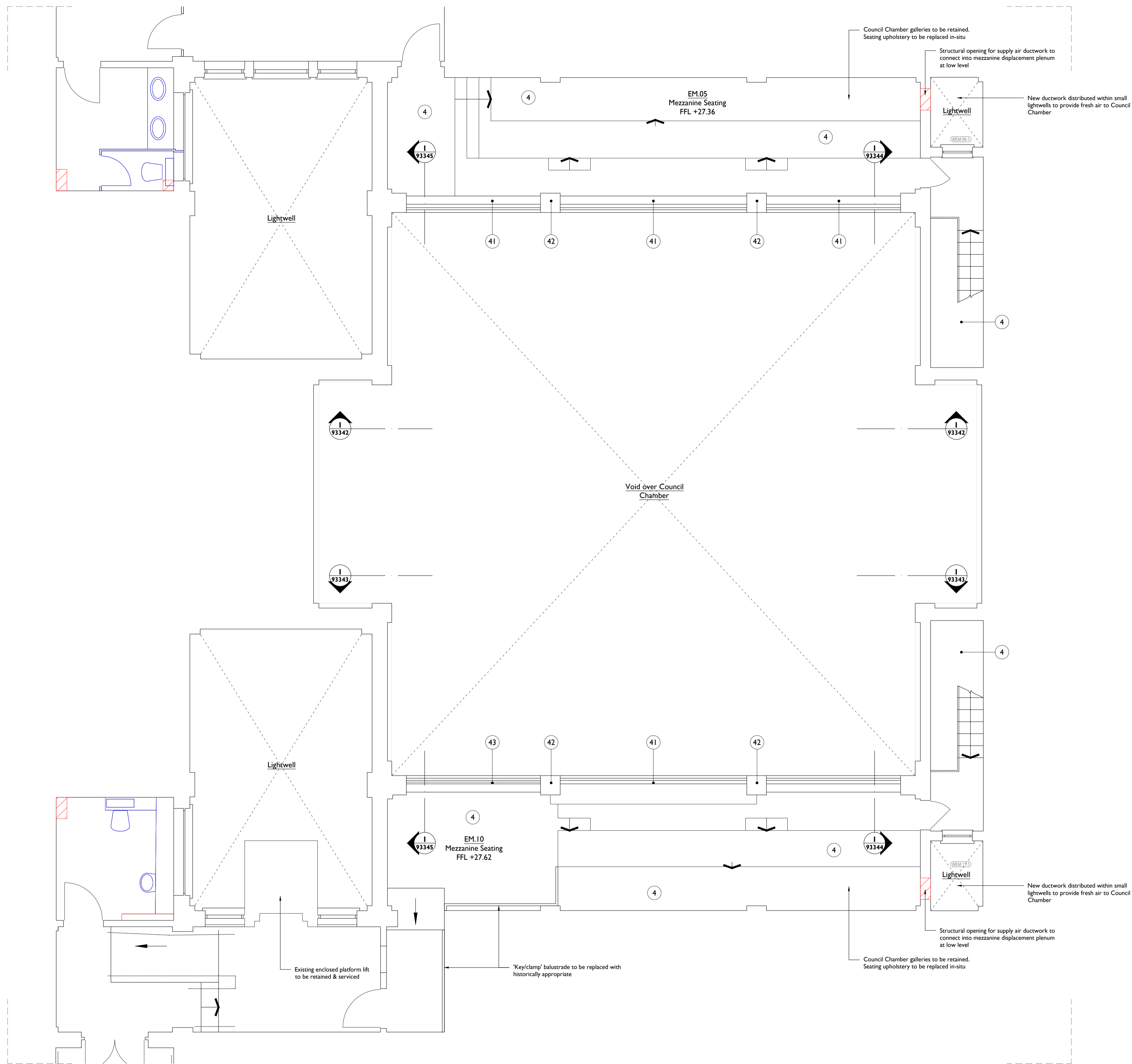
I EM.05 & EM.10 Existing Room Plan 93051 1:50 @ A1
