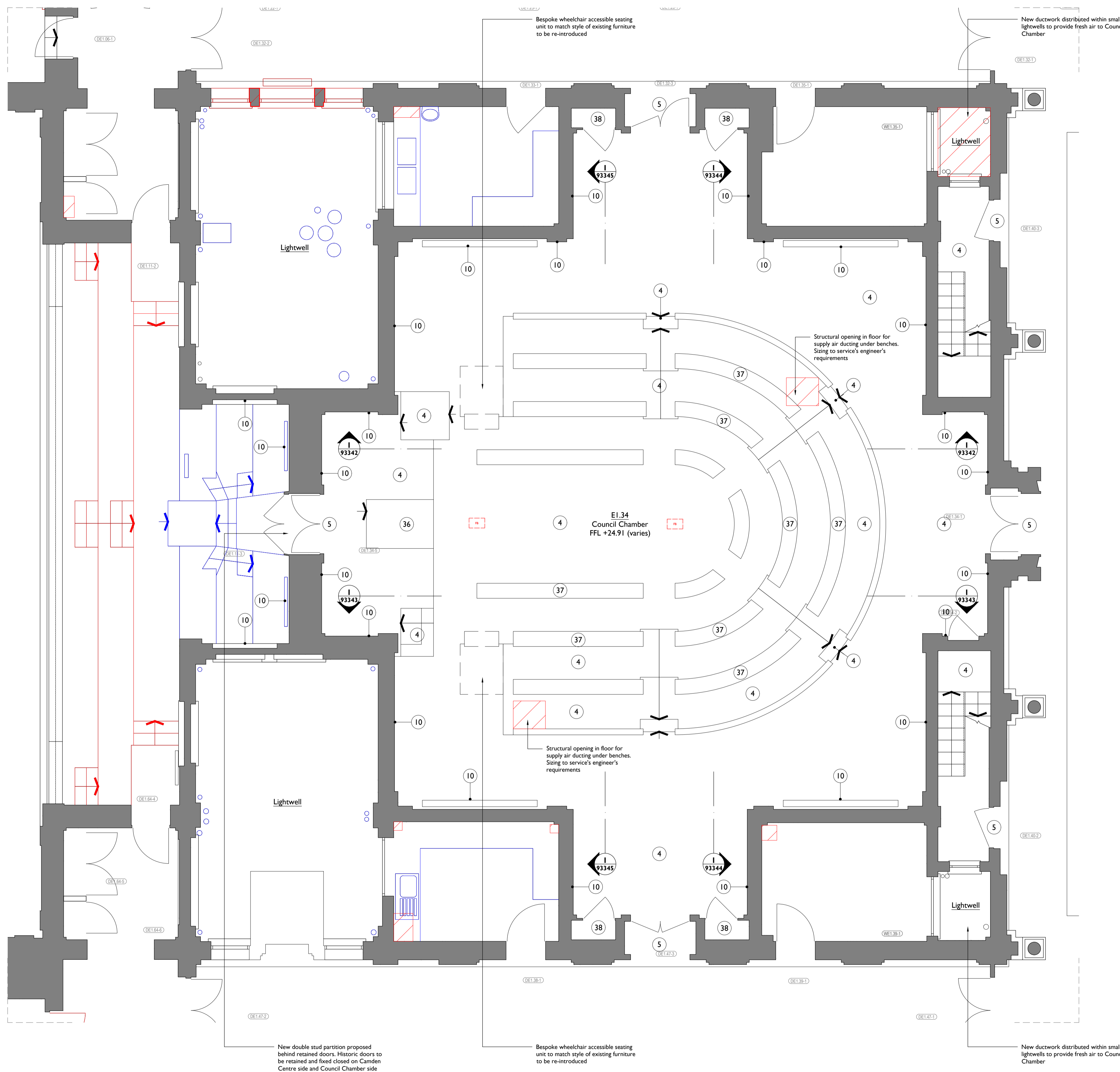
I E1.34 Existing Room Plan 93341 1:50 @ A1
