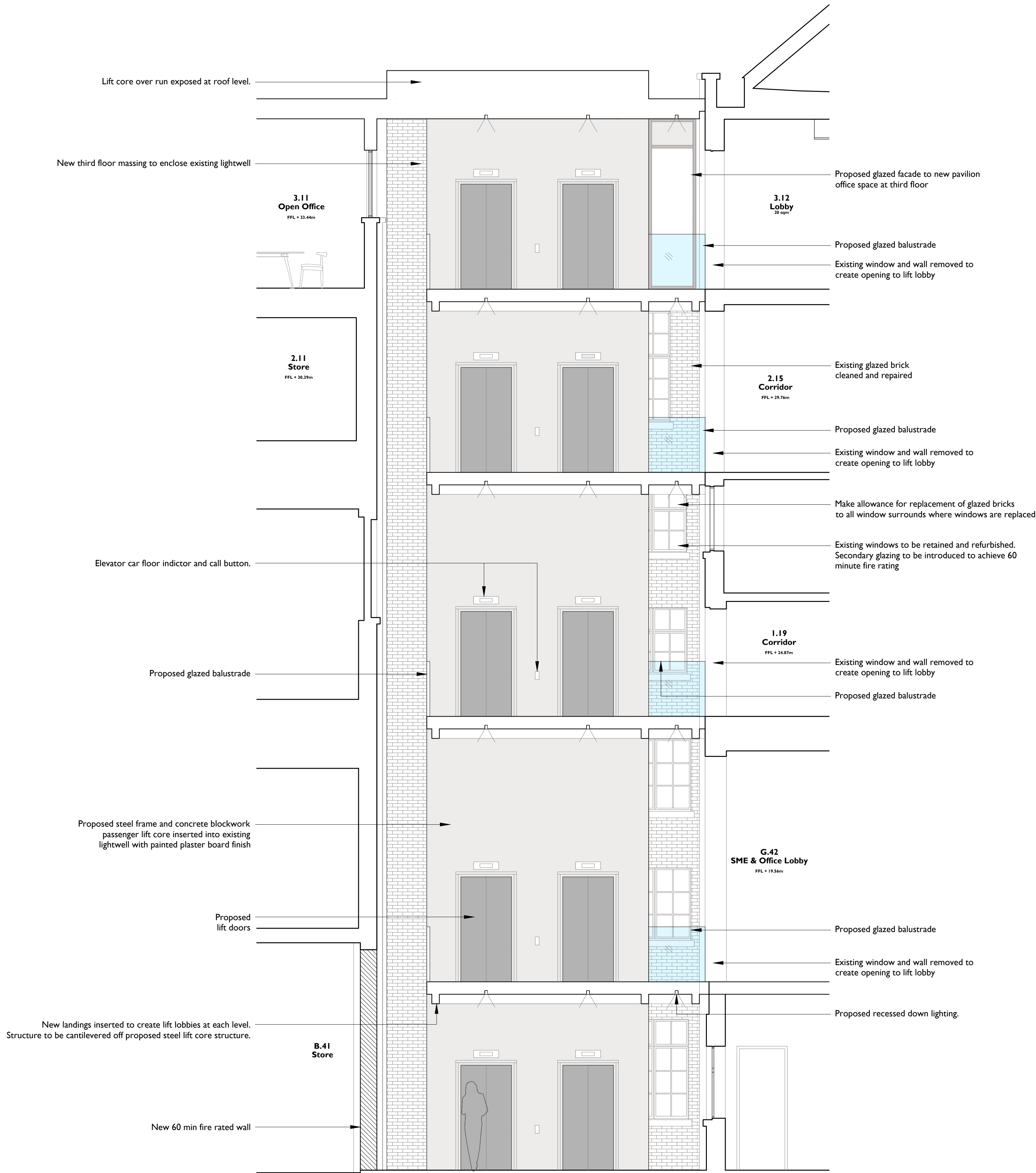
I SME OFFICE LIFT CORE SECTION AND PLAN 94015 1:50 @ A1
