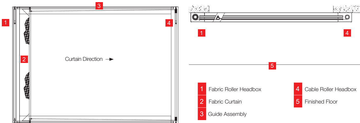
HORIZONTAL CURTAIN
